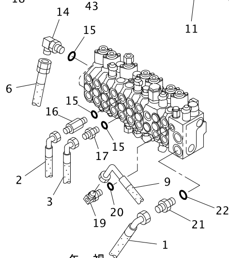
"A" 矢視 VIEW
