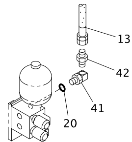
"C" 詳細 DETAIL
