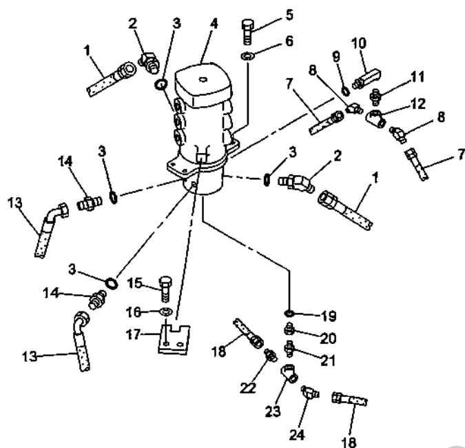
"A" 詳細 DETAIL
