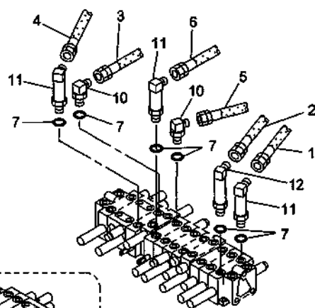
"C" 詳細 DETAIL
