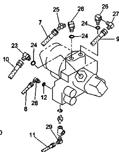
"C" 詳細 DETAIL
