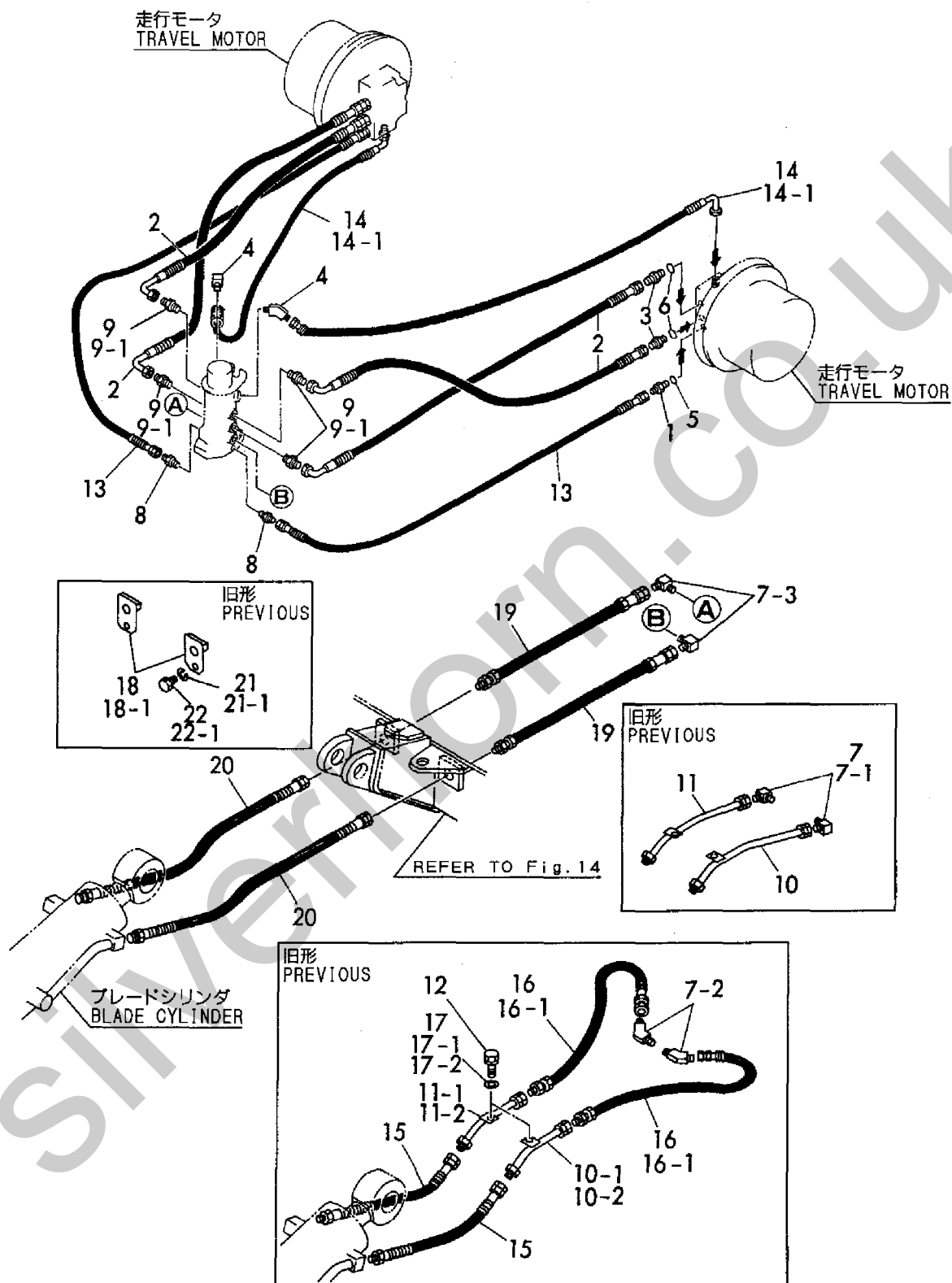
Fig. 62 油圧配管 (走行) HYD. OIL PIPING (TRAVEL)
