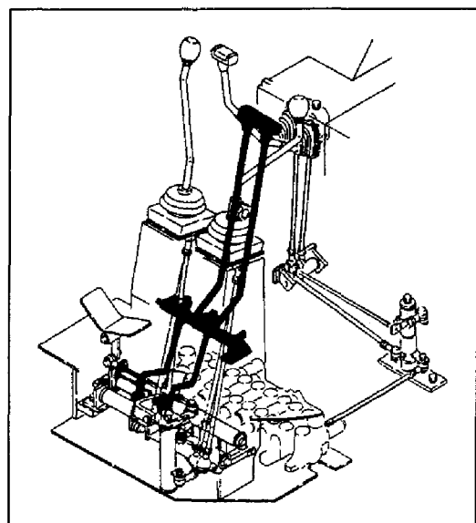
Fig. 26 操縦装置 (走行, マルチタイプ) CONTROL EQUIPMENT (TRAVEL, MULTI TYPE)
