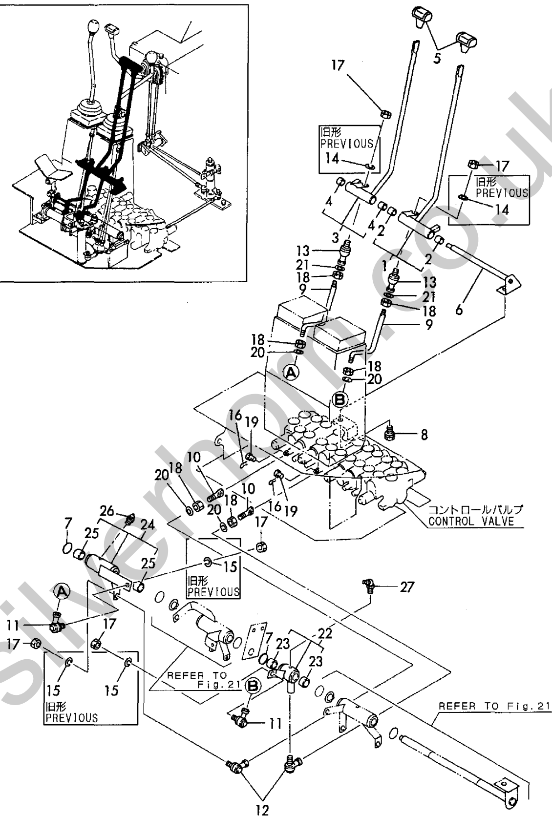
Fig. 26 操縦装置 (走行, マルチタイプ) CONTROL EQUIPMENT (TRAVEL, MULTI TYPE)
