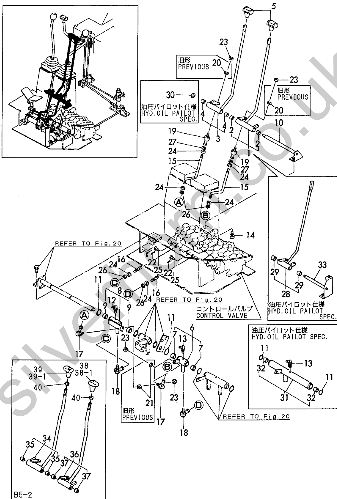
Fig. 25 操縦装置 (走行) CONTROL EQUIPMENT (TRAVEL)
