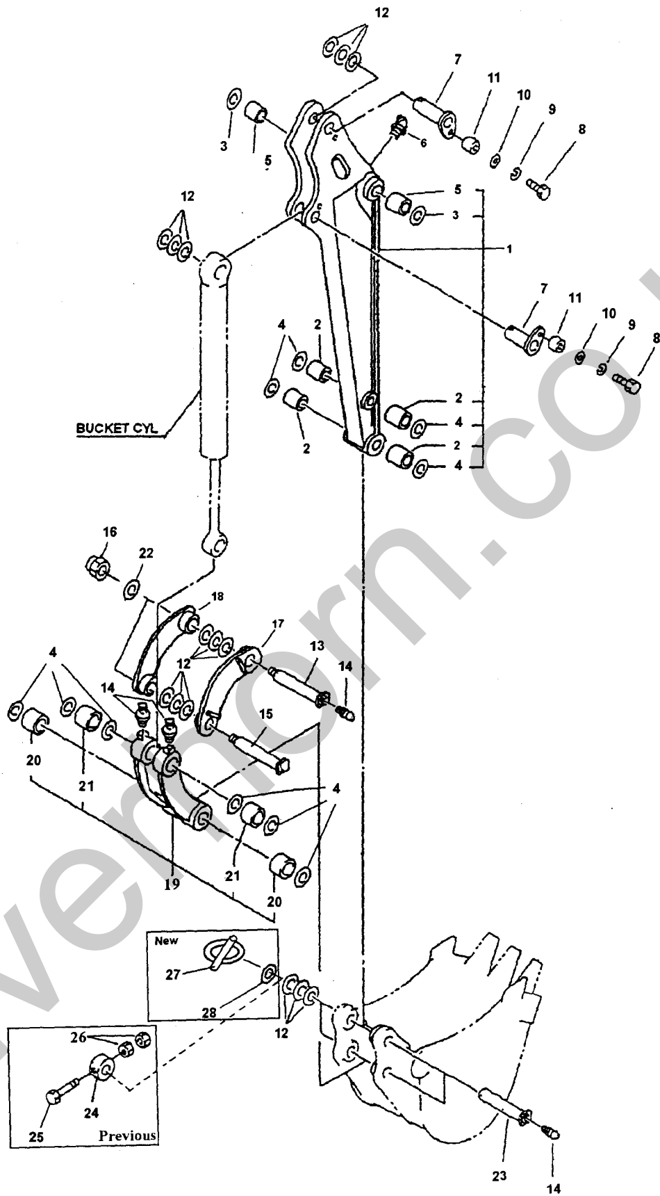
Fig 34 ARM & BUCKET LINK
