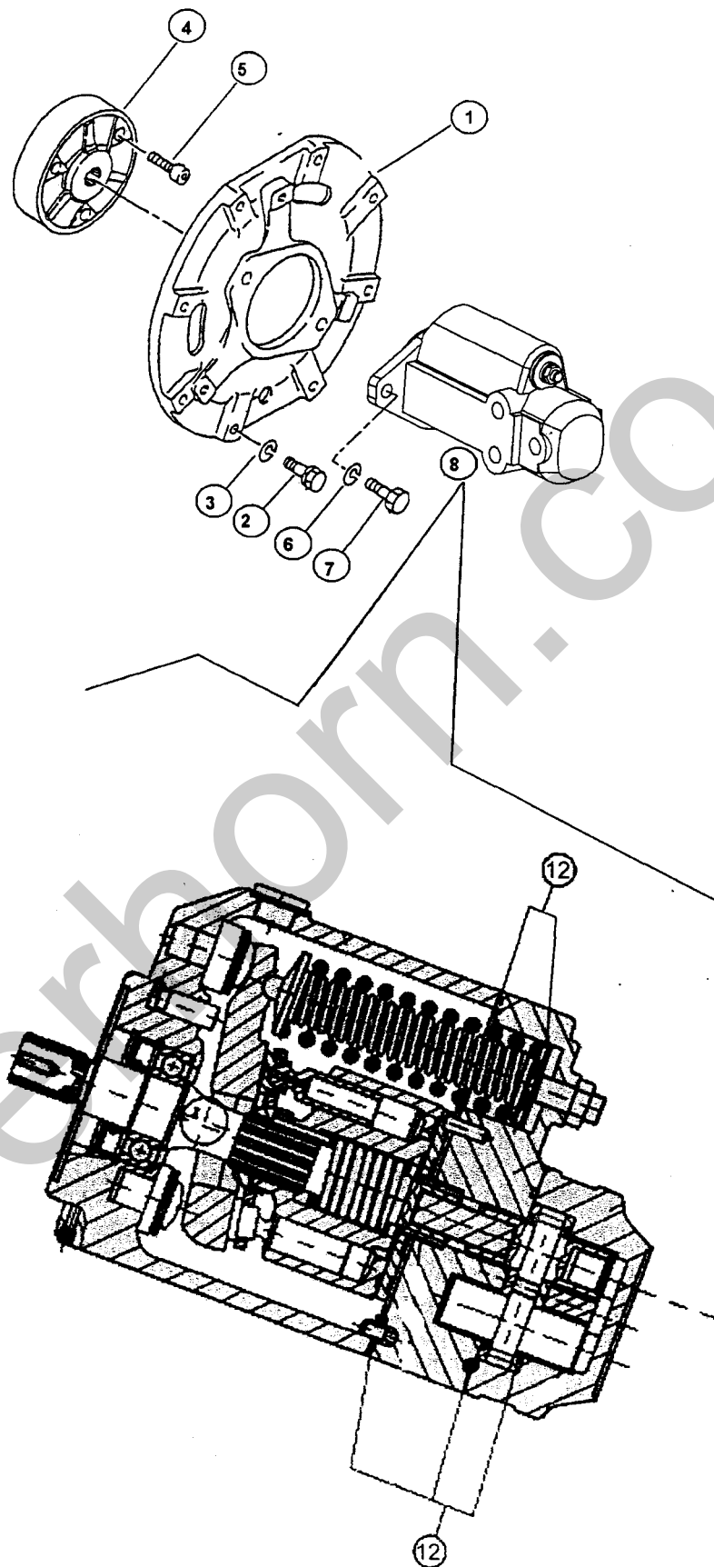
Fig 28 HYD OIL PUMP & JOINT
