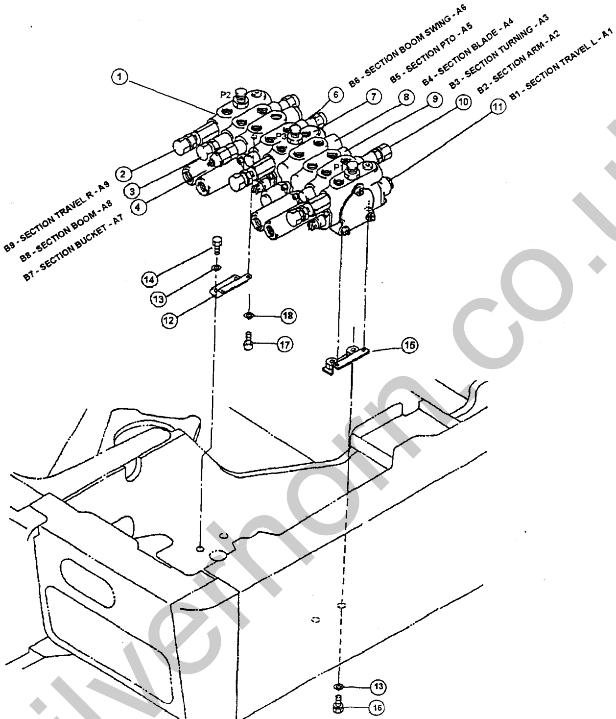
Fig 38 CONTROL VALVE
