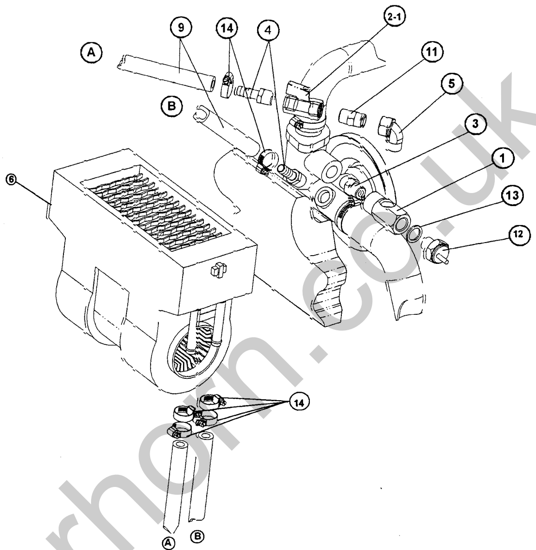
Fig 13 HEATER
