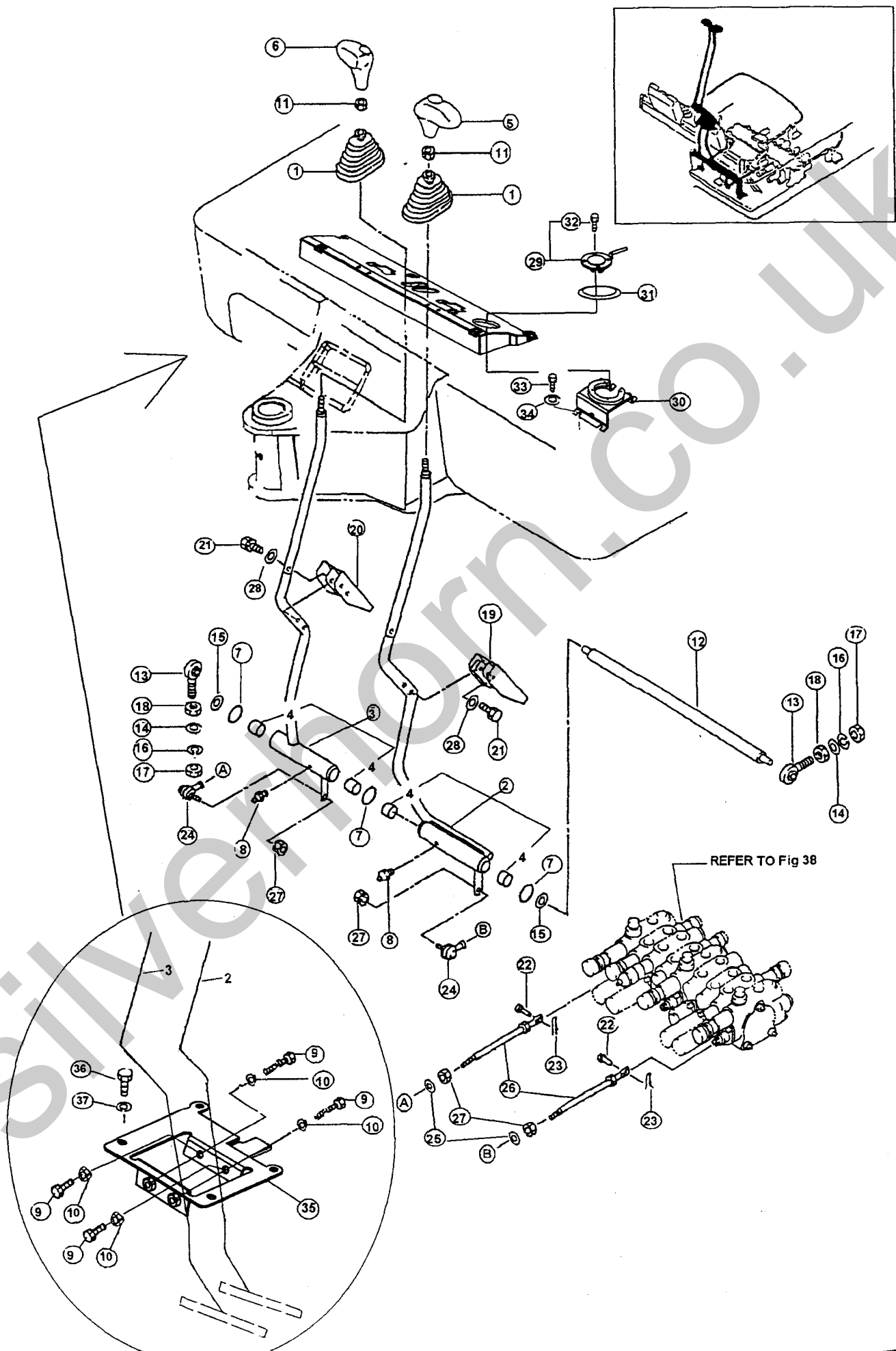
Fig 17 CONTROL EQUIPMENT (DRIVE)
