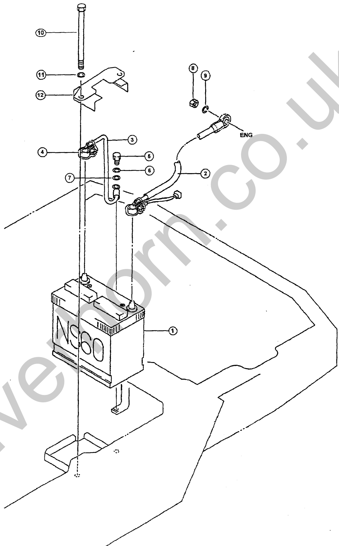
Fig 8 BATTERY
