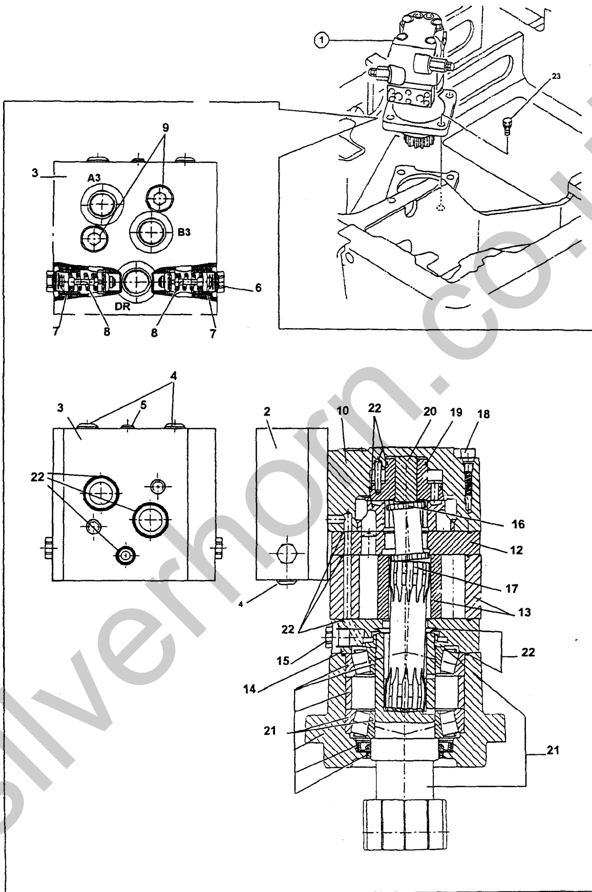
Fig 36 TURNING MOTOR
