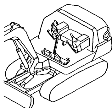
Fig. 71 リモコンバルブ (右: AS仕様) REMOTE CONTROL VALVE (RIGHT: AS SPEC.)
