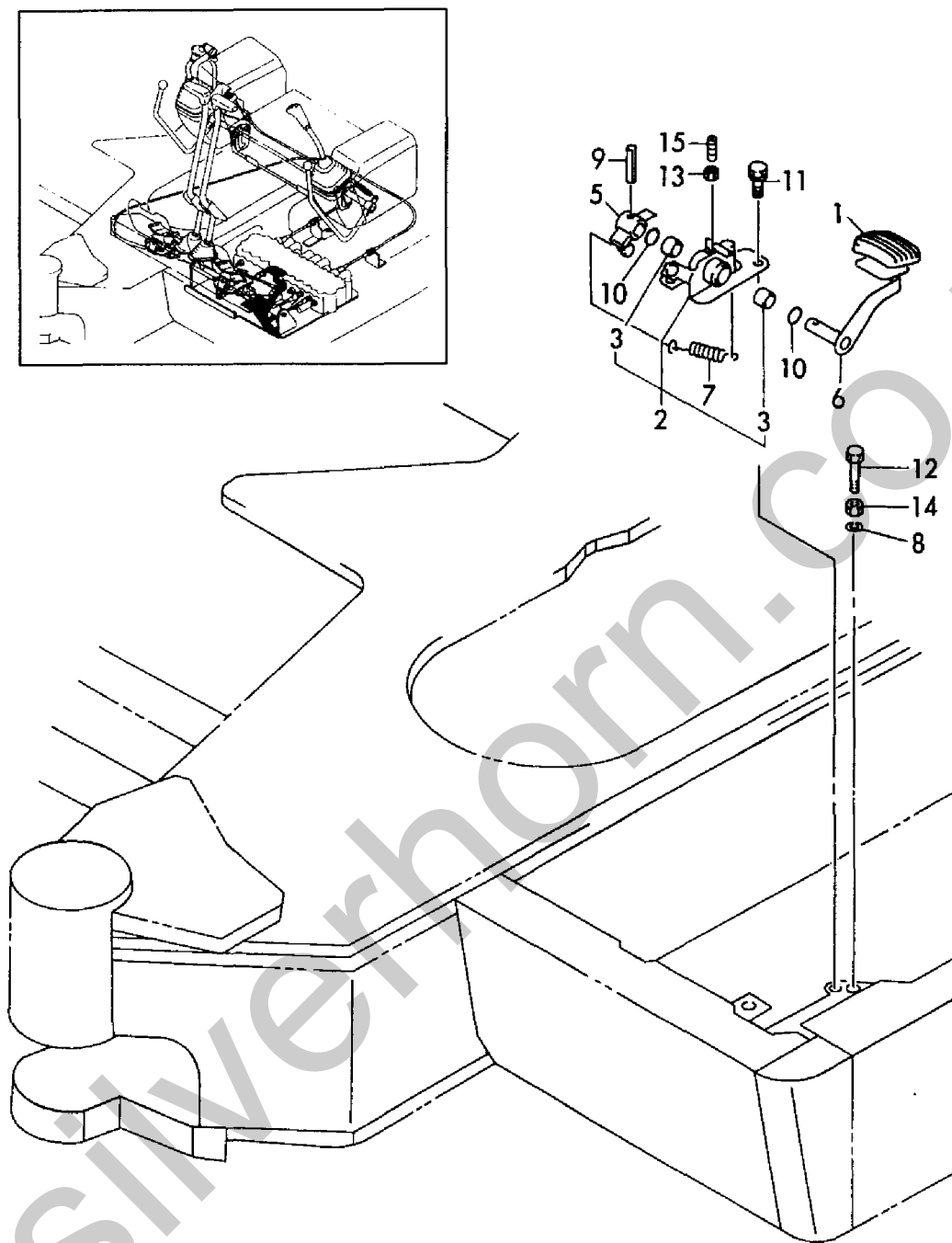
Fig. 35 操縦装置 (ローハイペダル) CONTROL EQUIPMENT (LOW-HIGH PEDAL)
