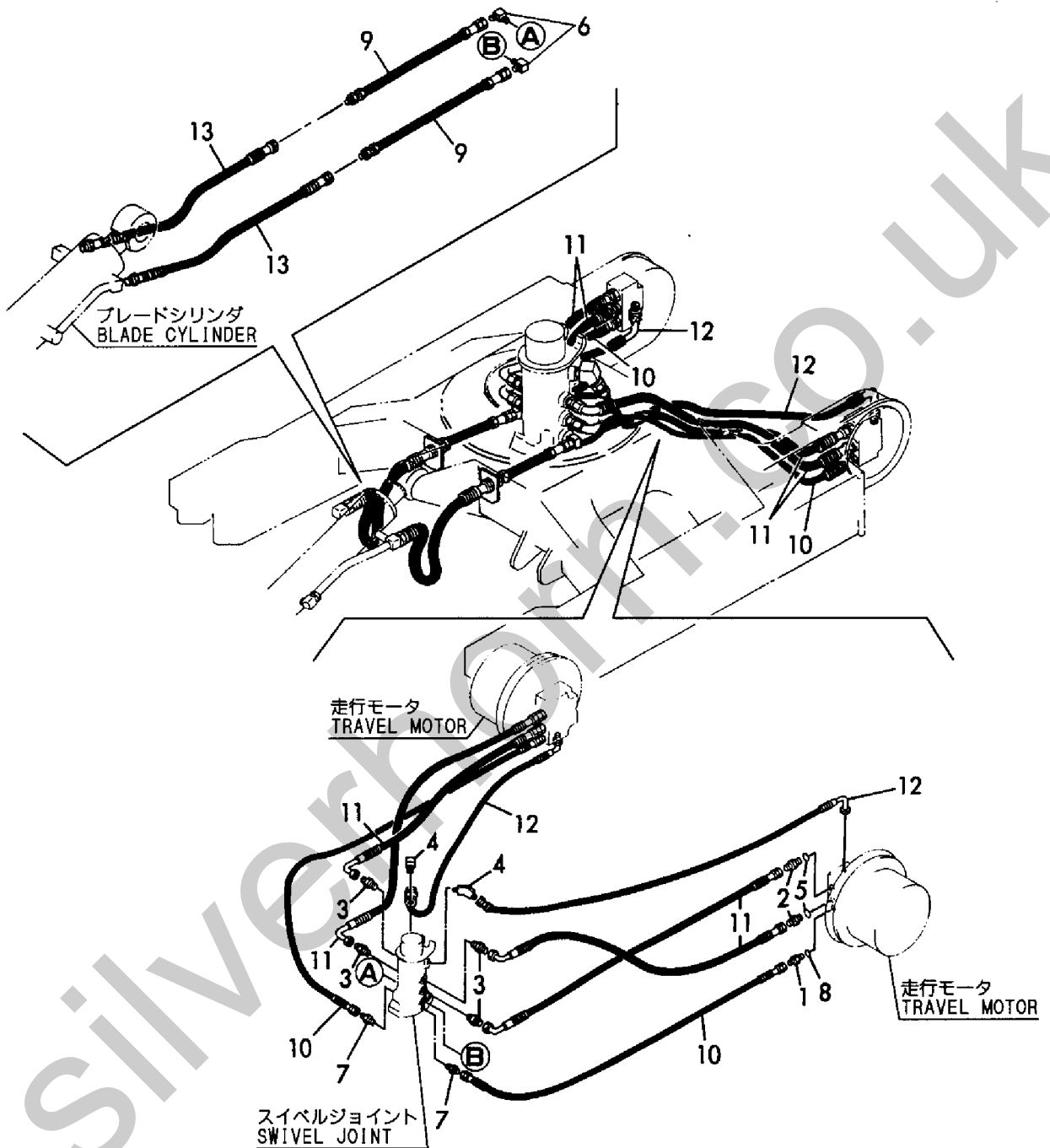
Fig. 86 油圧配管 (走行) HYD. OIL PIPING (TRAVEL)
