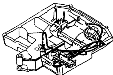
Fig. 86 油圧配管 (走行) HYD. OIL PIPING (TRAVEL)
