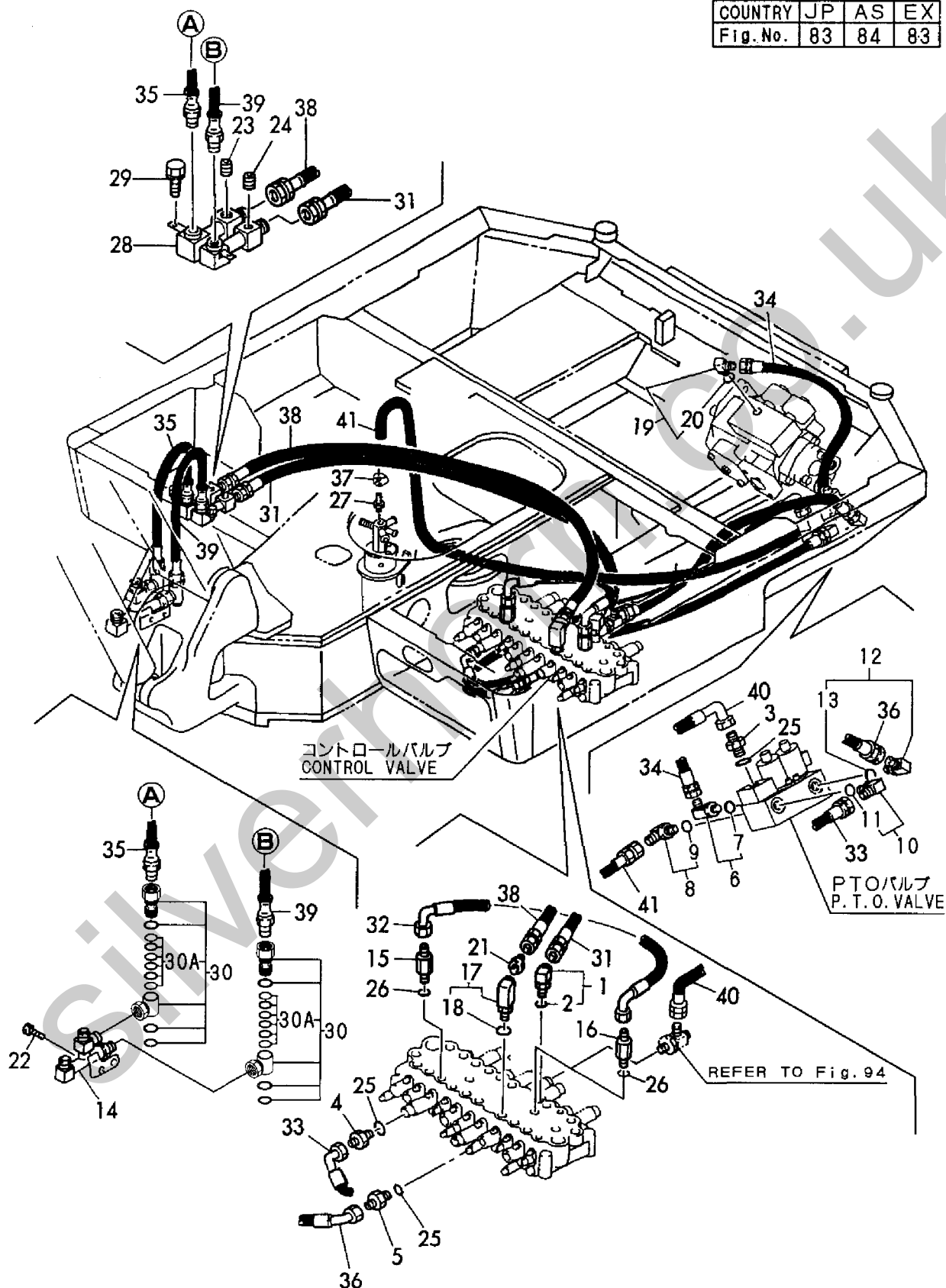
Fig. 84 油圧配管 (PTOバルブ/フレーム) (AS) HYD. OIL PIPING (P. T. O. VALVE/FRAME) (AS)
