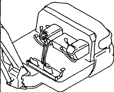
Fig. 74 リモコンバルブ (左) (AS) REMOTE CONTROL VALVE (LEFT) (AS)
