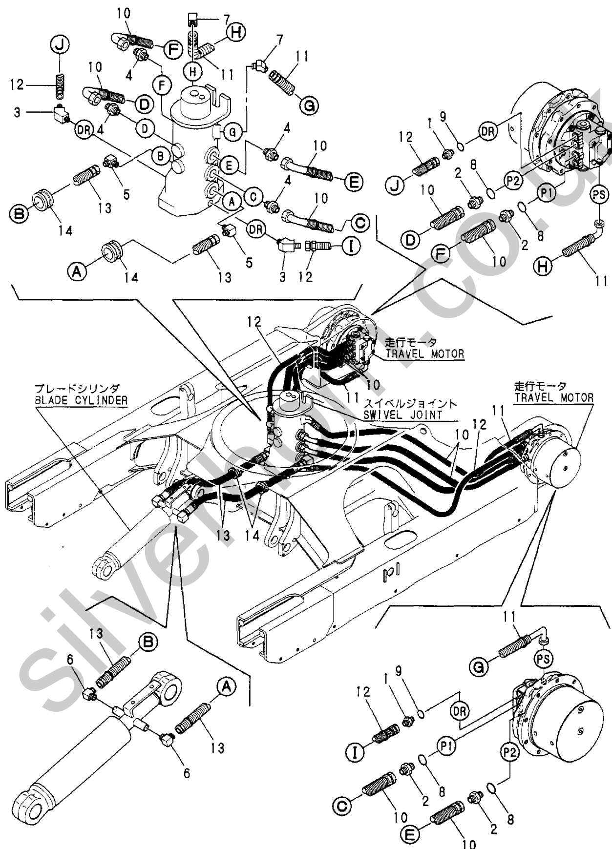
Fig. 82 油圧配管 (走行) HYD. OIL PIPING (TRAVEL)
