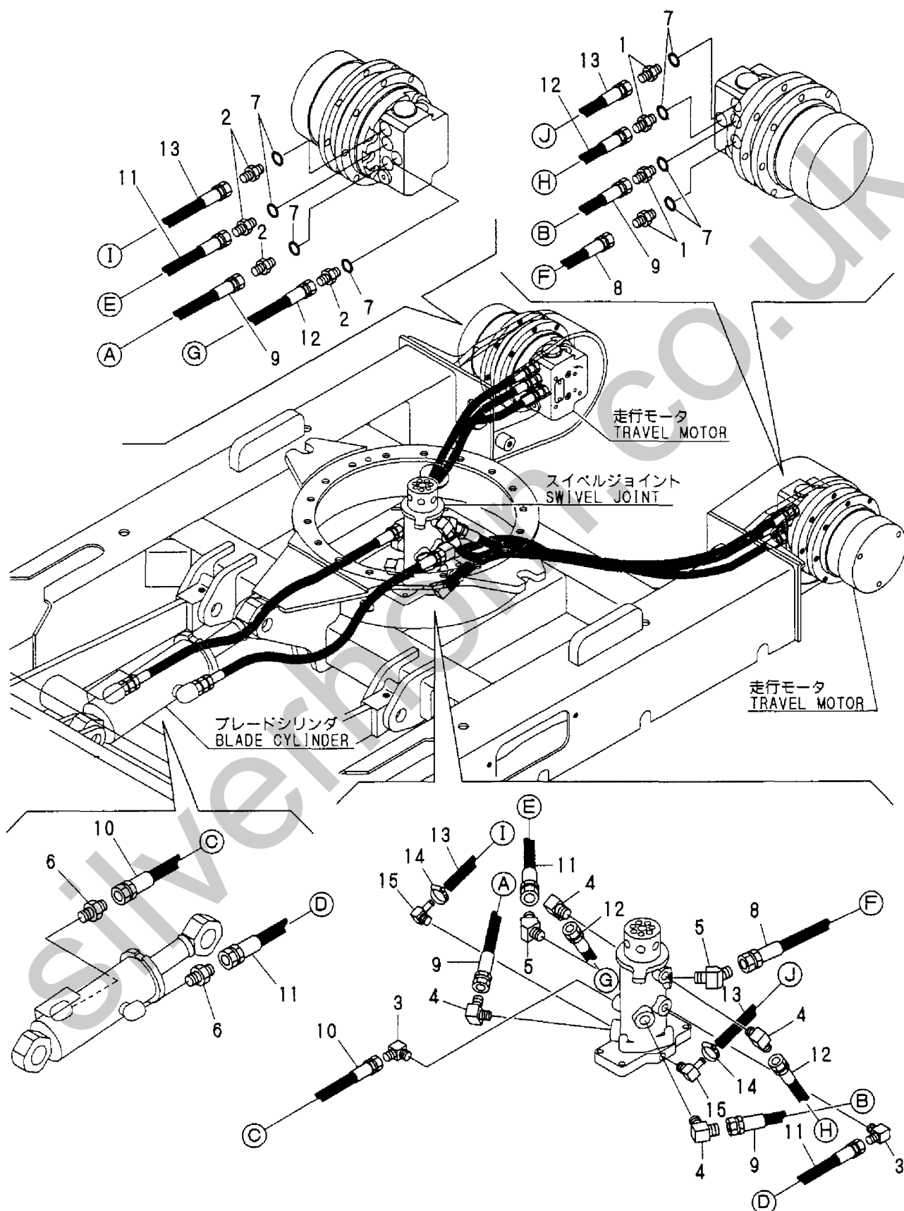
Fig. 39 油圧配管 (走行) HYD. OIL PIPING (TRAVEL)
