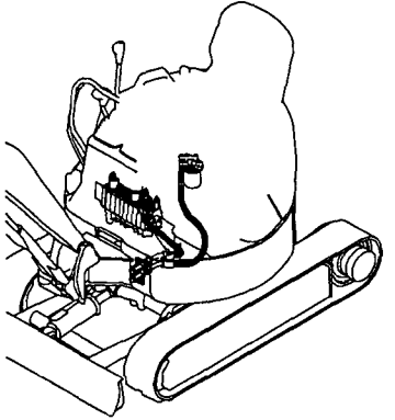
Fig. 39 油圧配管 (走行) HYD. OIL PIPING (TRAVEL)
