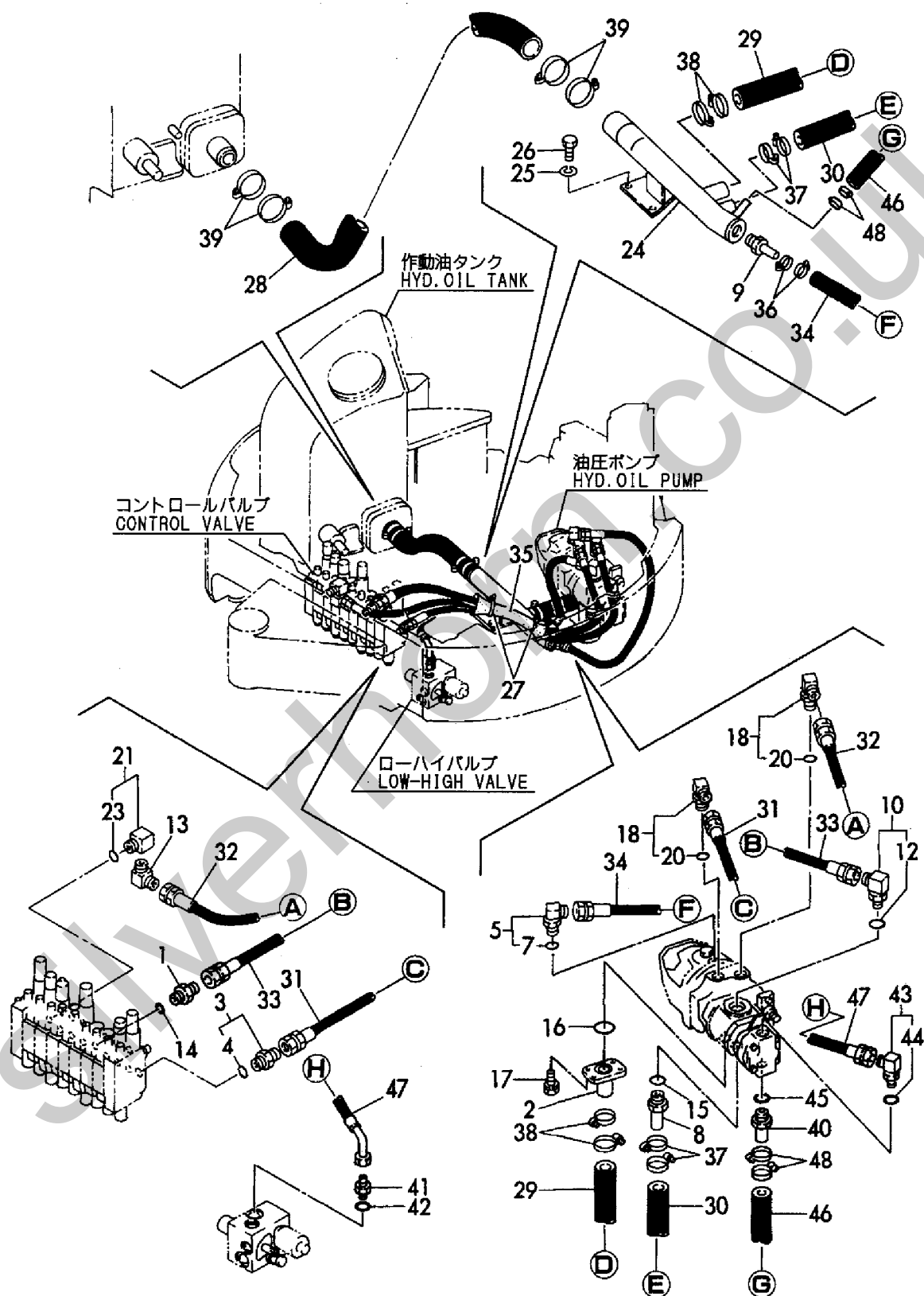
Fig. 43 油圧配管 (タンク~ポンプ~バルブ) (旧形) HYD. OIL PIPING (TANK~PUMP~VALVE) (PREVIOUS) ~M/#03463, 03466
