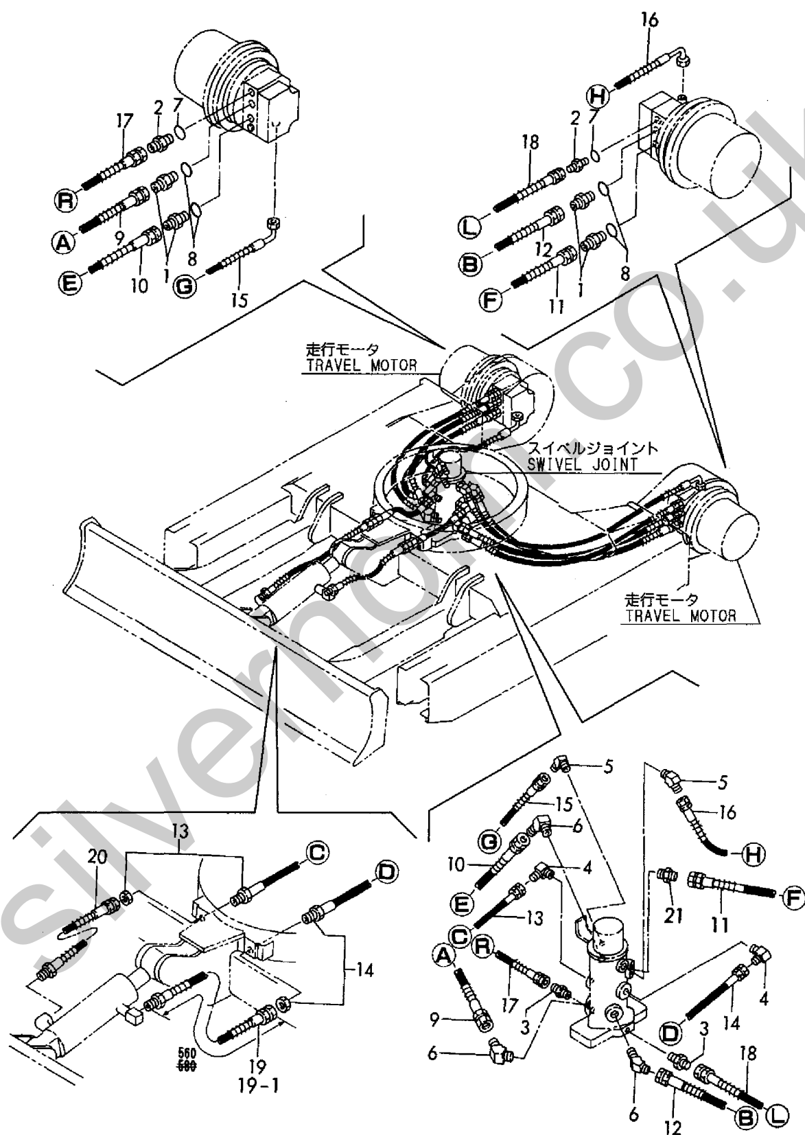
Fig. 49 油圧配管 (走行) HYD. OIL PIPING (TRAVEL)
