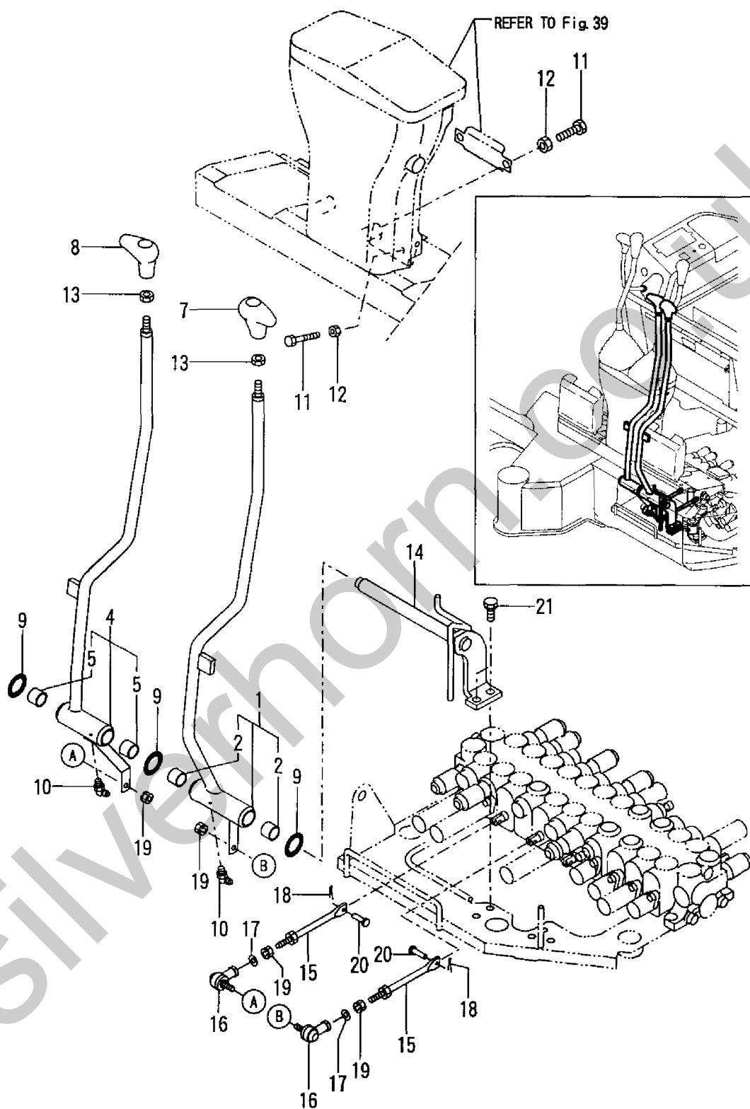
Fig. 40 操縦装置(走行) CONTROL EQUIPMENT(DRIVE)
