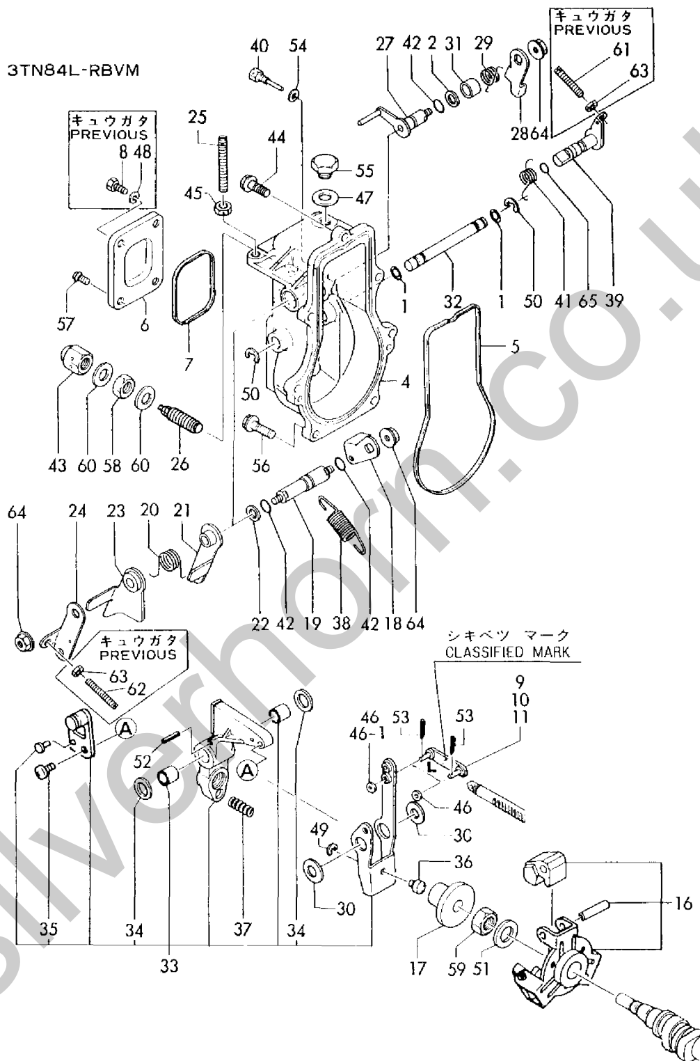
Fig. 23 ガバナ GOVERNOR
