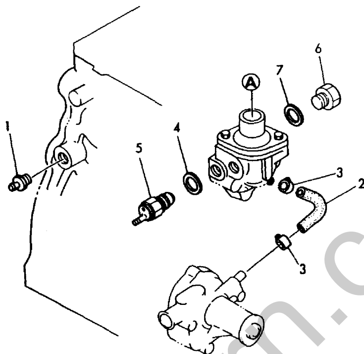
Fig. 15 CWパイプ COOLING WATER LINE
