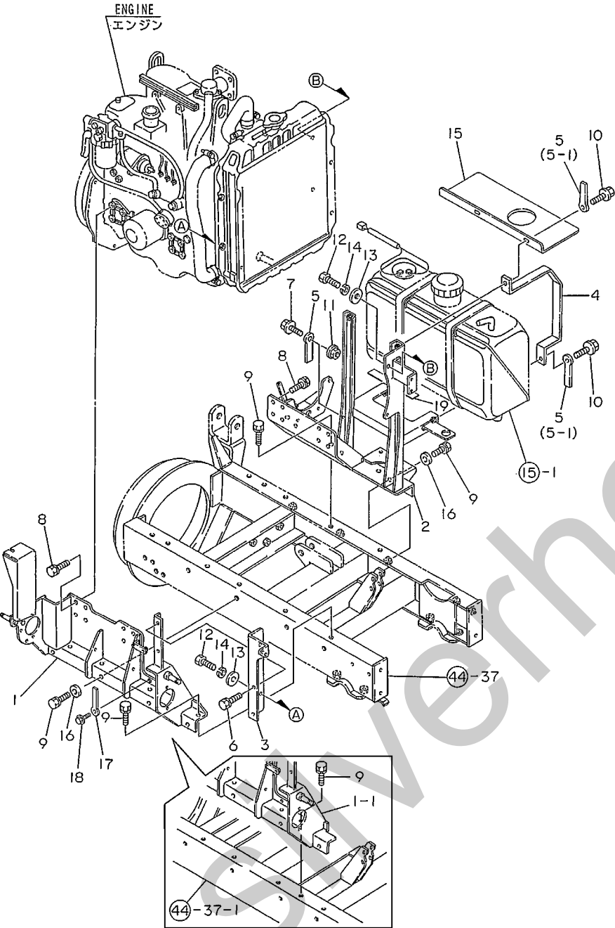
Fig.40. ENGINE MOUNTING
