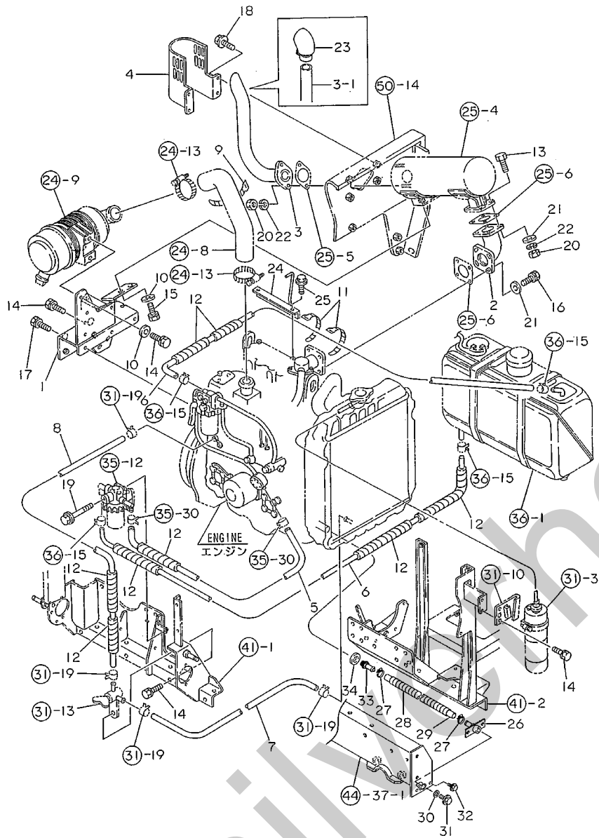
Fig.43. ENGINE RELATED
