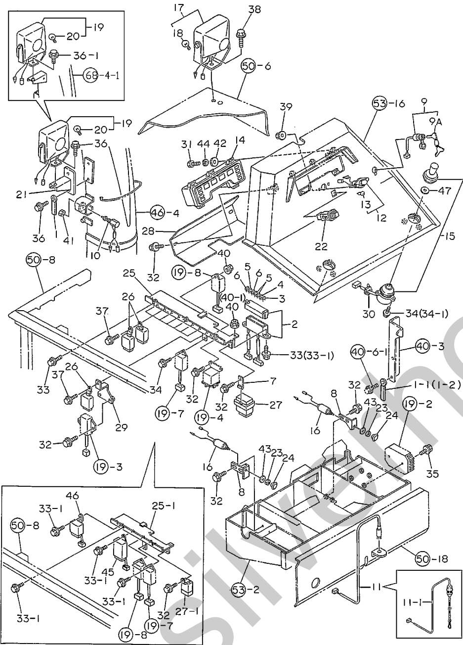
Fig.56. ELECTRICAL PARTS
