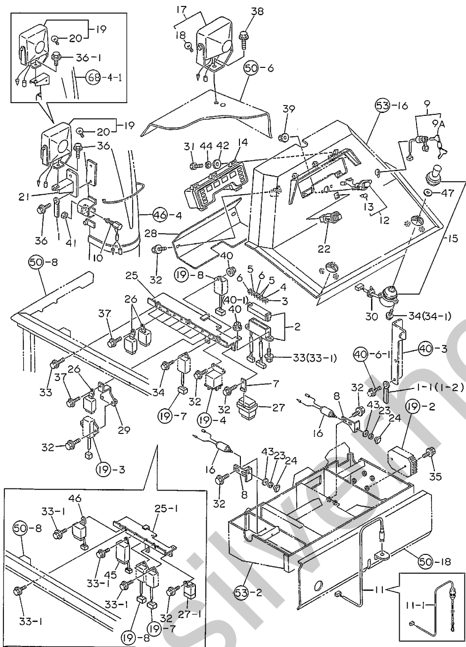
Fig.56. ELECTRICAL PARTS
