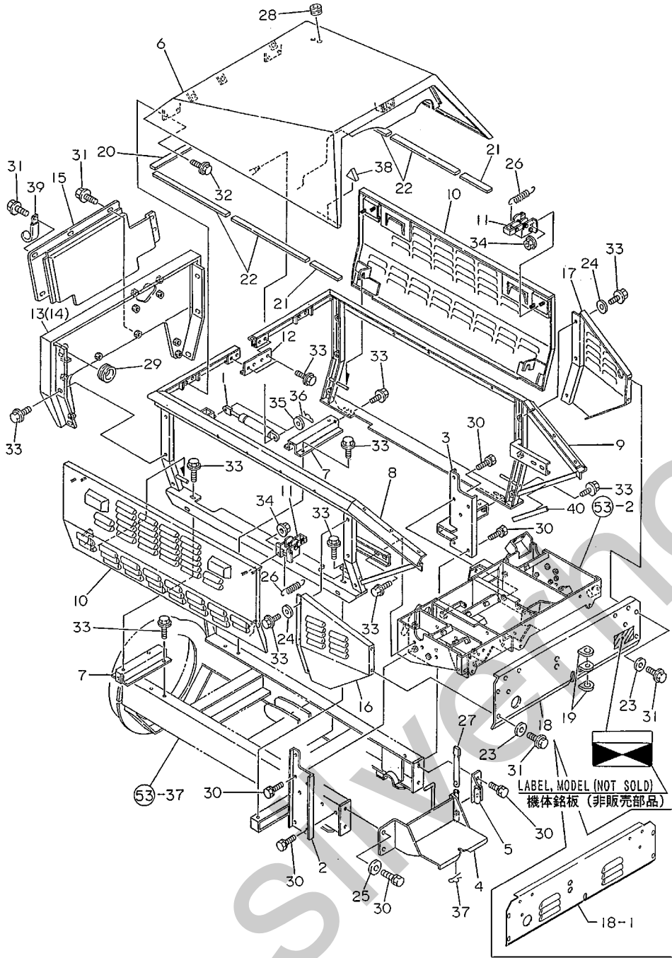
Fig.50. COVERS
