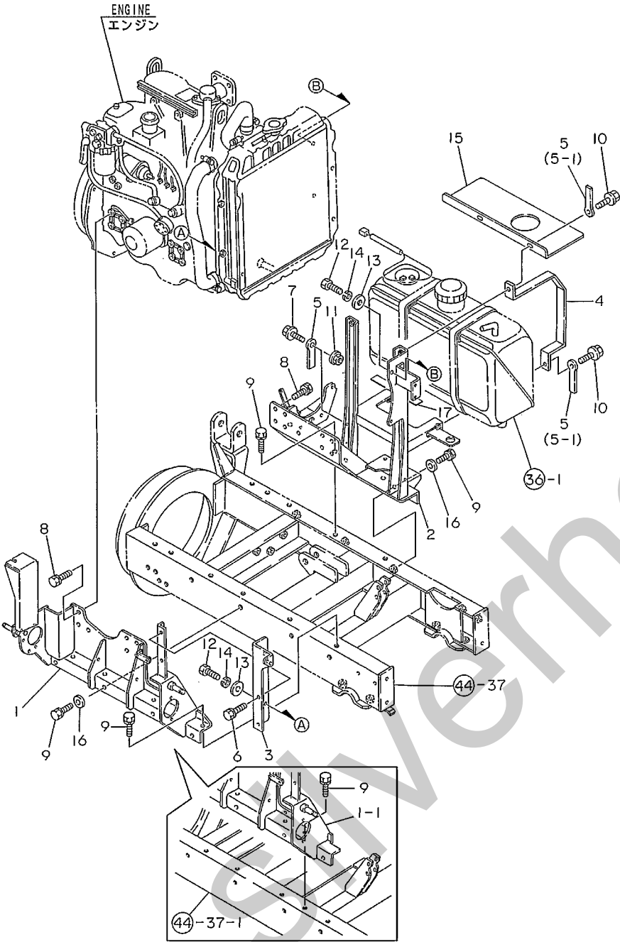
Fig.41. ENGINE MOUTING
