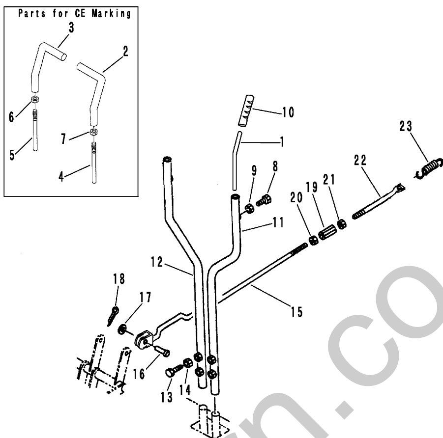
FIG 10 SIDE CLUTCH LEVER
