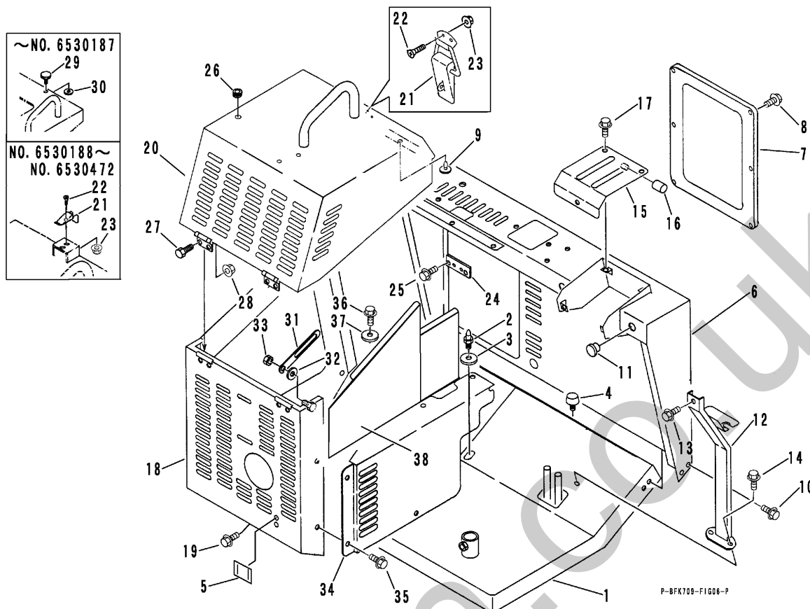
FIG 6 FRAME &amp; ENGINE COVER (DIESEL)
