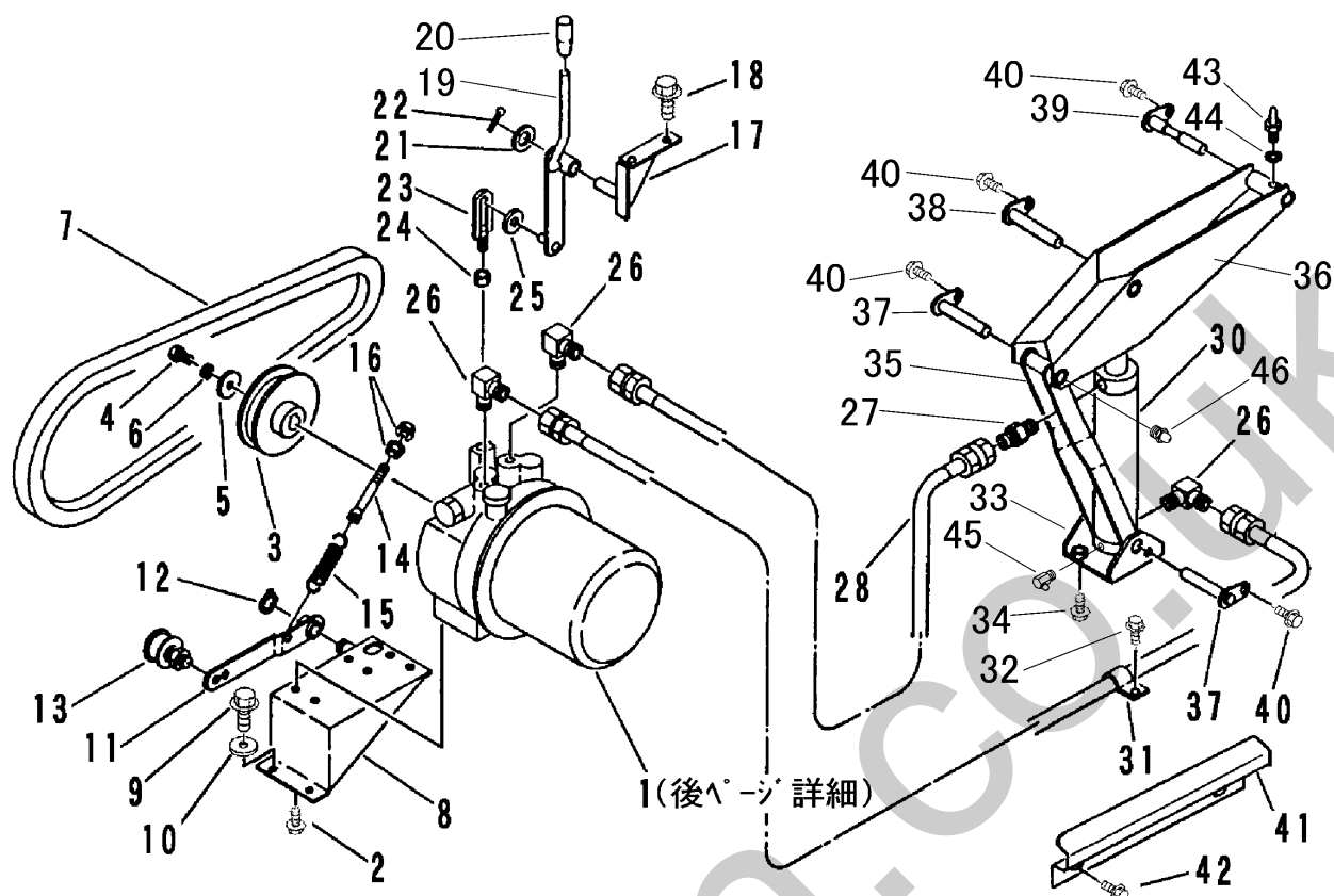
FIG 15 HYDRAULIC LINE
