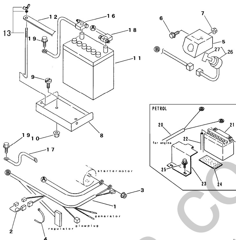
FIG 3 ELECTRIC EQUIPMENT
