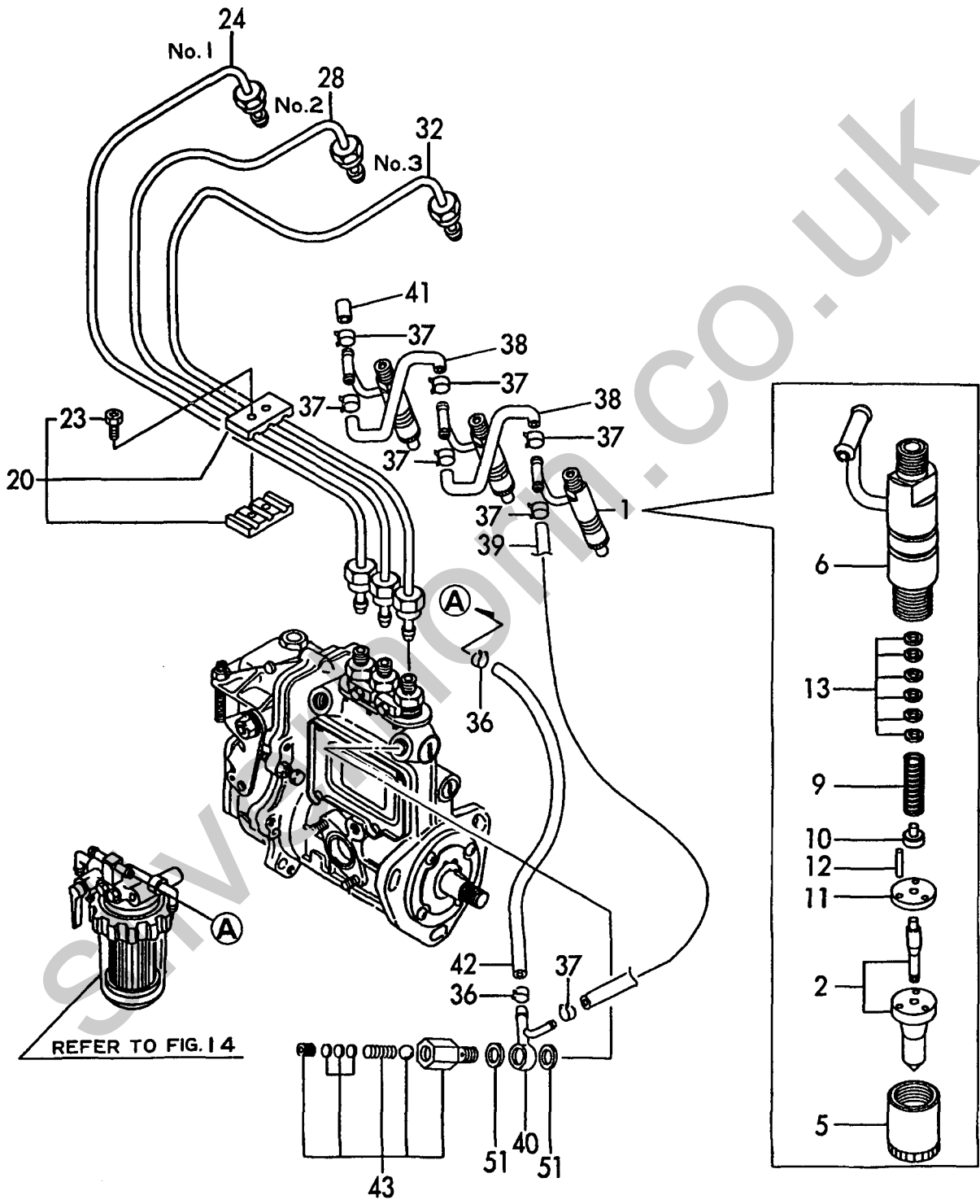
Fig. 13 燃料噴射弁 FUEL INJECTION VALVE
