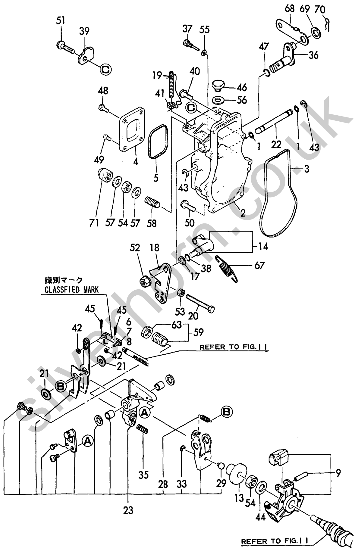
Fig. 12 ガバナ GOVERNOR
