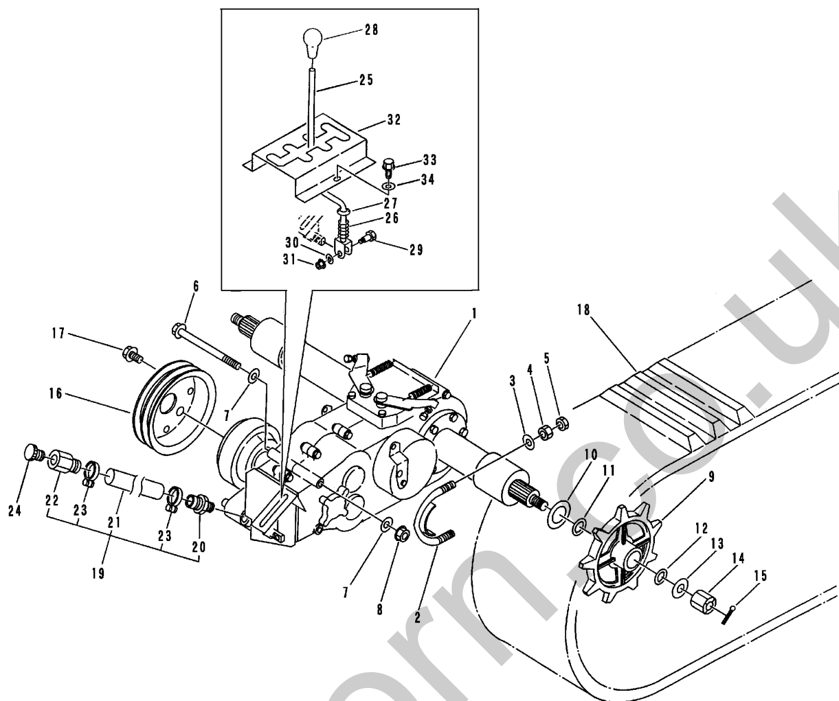
TRANSMISSION &amp; GEAR SHIFT
