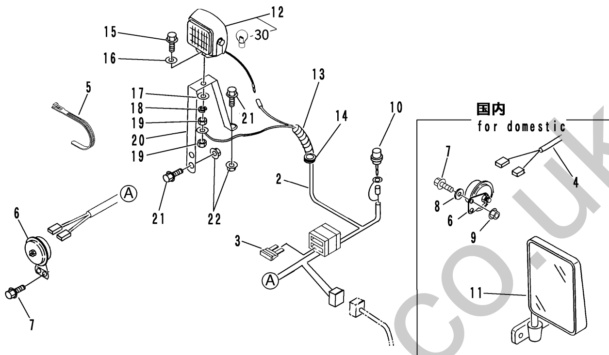
FIG 6 デンソウ (ソノ3) ELECTRIC EQUIPMENT (PART-3)
