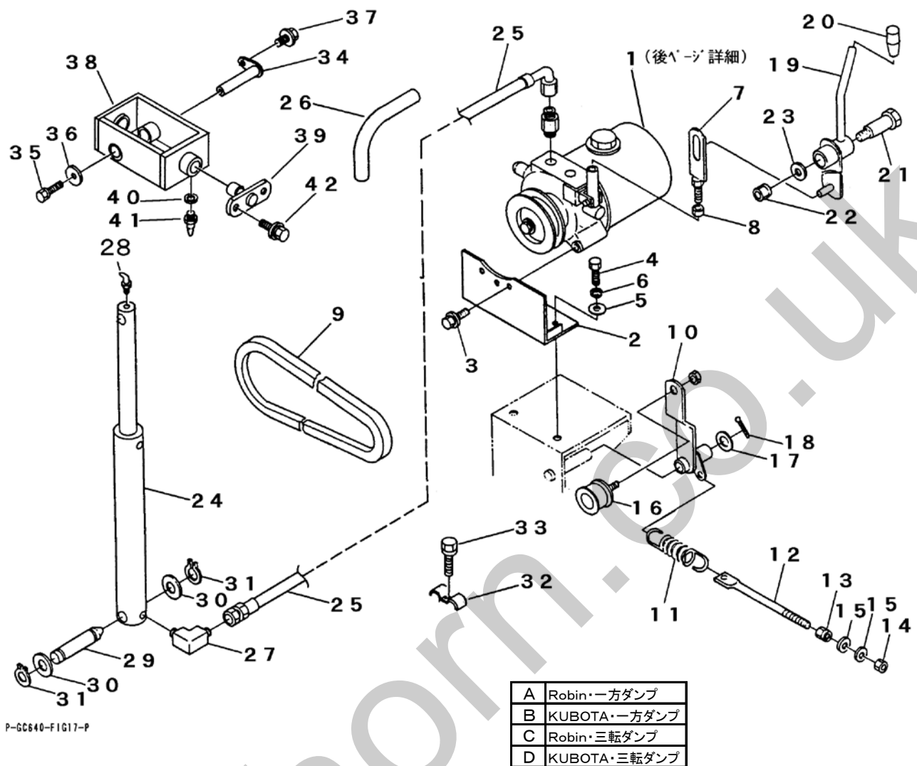
FIG 17 ユアツ HYDRAULIC EQUIPMENT
