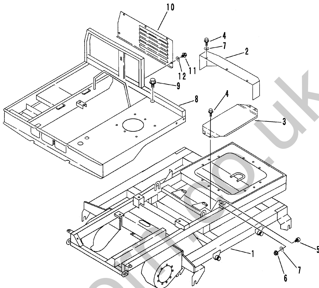
CHASSIS &amp; SUB CHASSIS (SLEWING &amp; DUMPING)
