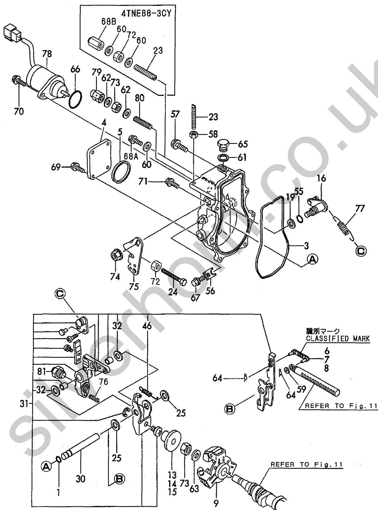
Fig. 12 ガバナ GOVERNOR
