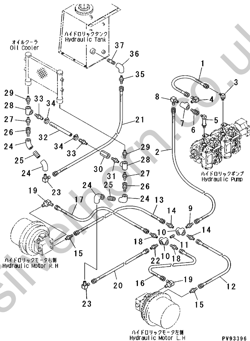
FIG.505A HYDRAULIC PIPING (OIL COOLER AND RETURN LINE) (SERIAL NO. 60577-60650)
