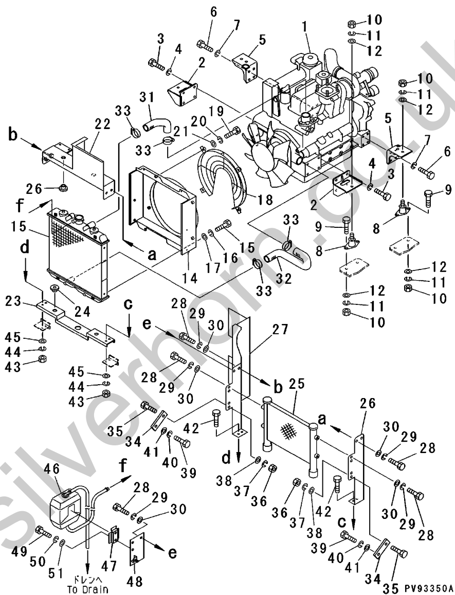
FIG.101 ENGINE RELATED PARTS (ENGINE MOUNTING PARTS AND RADIATOR) (SERIAL NO. 60501-60650)
