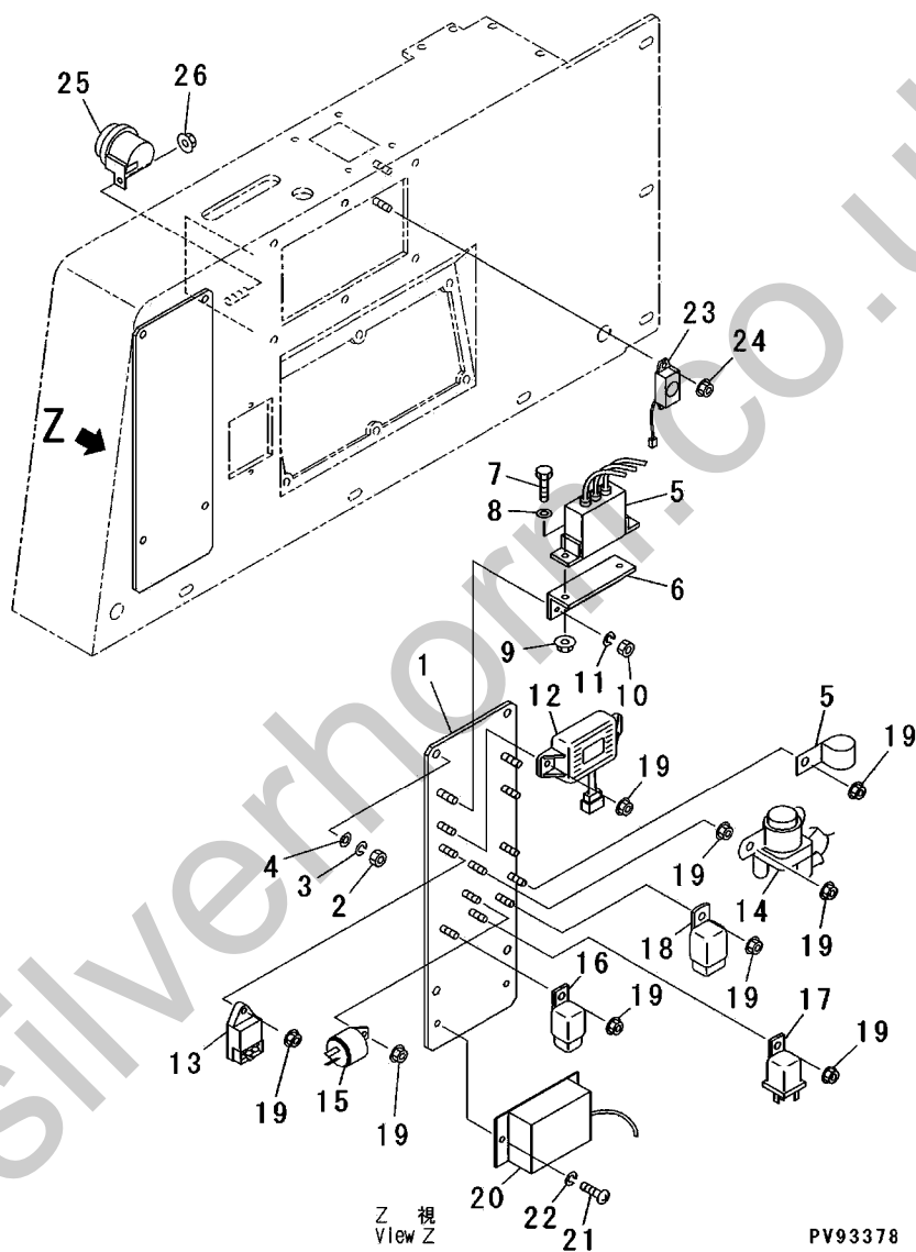
FIG.705 ELECTRICAL SYSTEM (RELAYS AND FUSE BOX) (SERIAL NO. 60501-60650)
