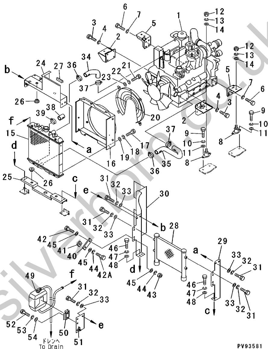
FIG.101A ENGINE RELATED PARTS (ENGINE MOUNTING PARTS AND RADIATOR) (SERIAL NO. 60651-)
