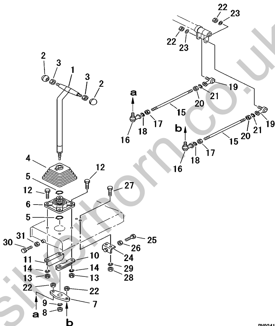
FIG.401 STEERING CONTROL SYSTEM (1/2) (SERIAL NO. 60501-60650)
