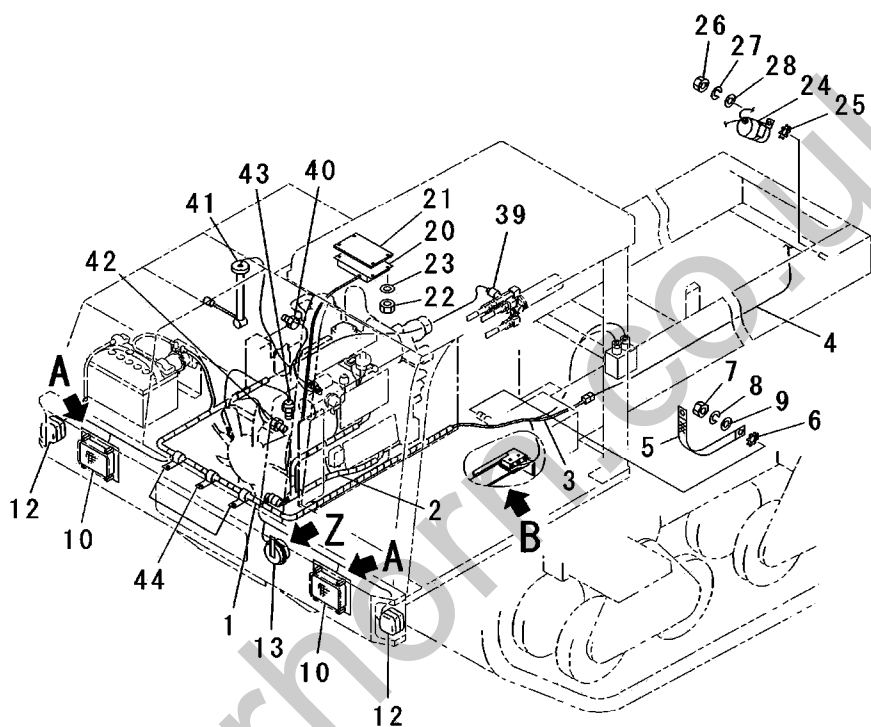
FIG.711A ELECTRICAL SYSTEM (1/4) (WIRING HARNESS AND LAMPS) (SERIAL NO. 60651-)
