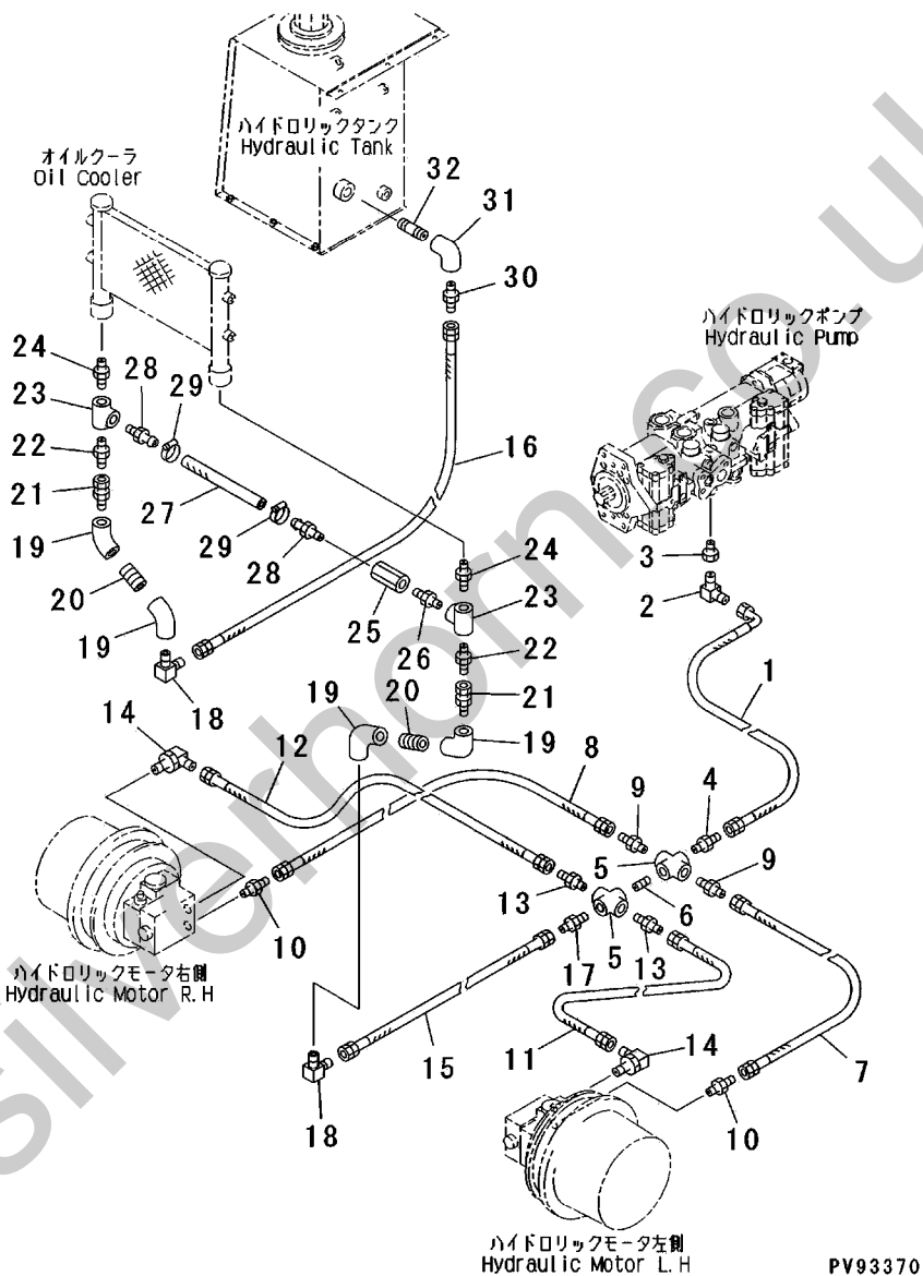
FIG.505 HYDRAULIC PIPING (OIL COOLER AND RETURN LINE) (SERIAL NO. 60501-60576)
