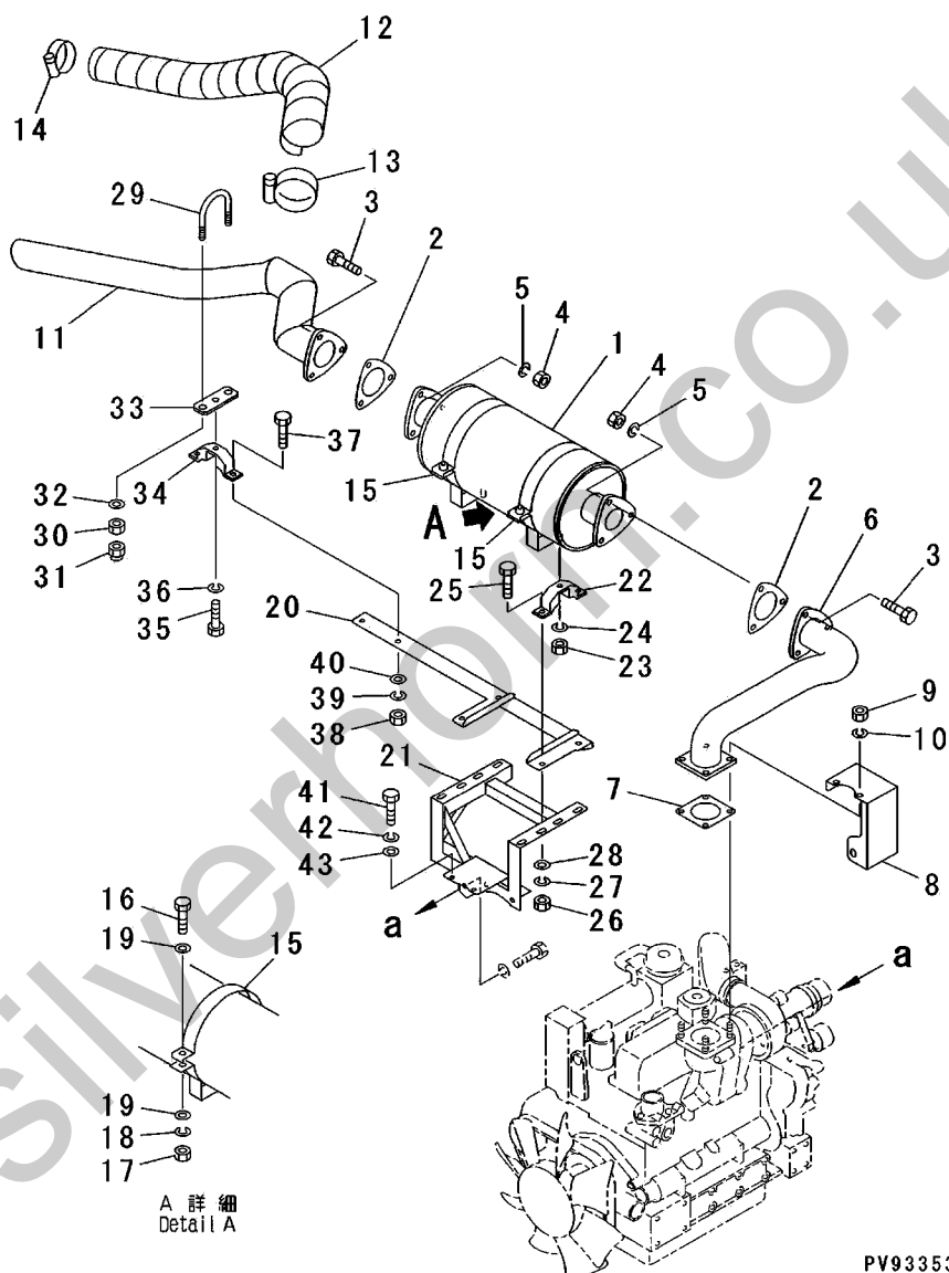
FIG.115 ENGINE RELATED PARTS (EXHAUST SYSTEM) (SERIAL NO. 60501-60583, 60585)
