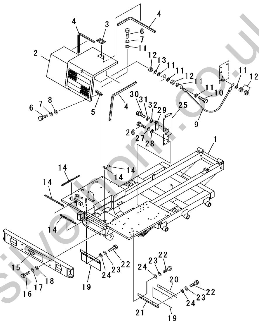
FIG.201A FRAME RELATED PARTS (1/5) (ENGINE BONNET AND FRONT BUMPER) (SERIAL NO. 60651-)
