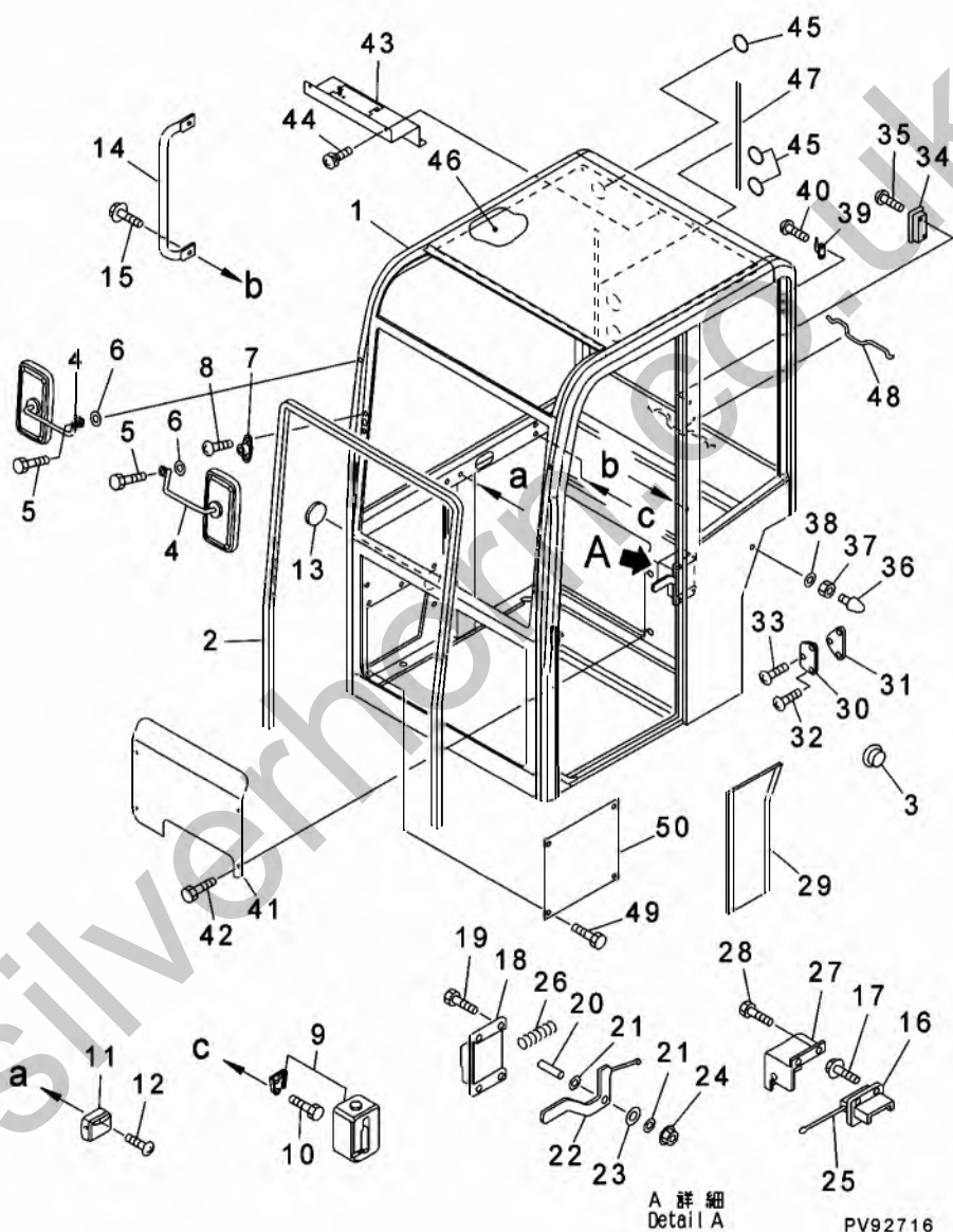
FIG. 223 CAB ASS'Y (1/3) (CAB AND RELATED PARTS) (APPLICABLE TO CAB SPEC.)
