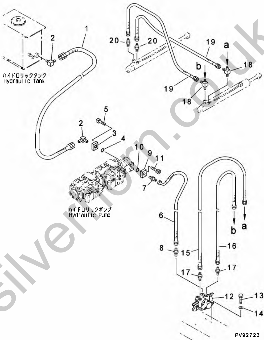
FIG. 501 HYDRAULIC PIPING (CONTROL VALVE AND DUMP CYLINDER LINE)
