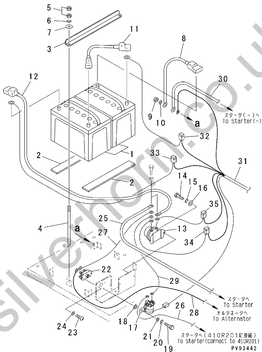
FIG..715 ELECTRICAL SYSTEM (BATTERY AND BATTERY RELAY)
