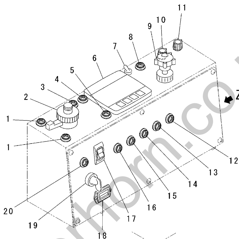
FIG..701 ELECTRICAL SYSTEM (CONTROL PANEL BOX)
