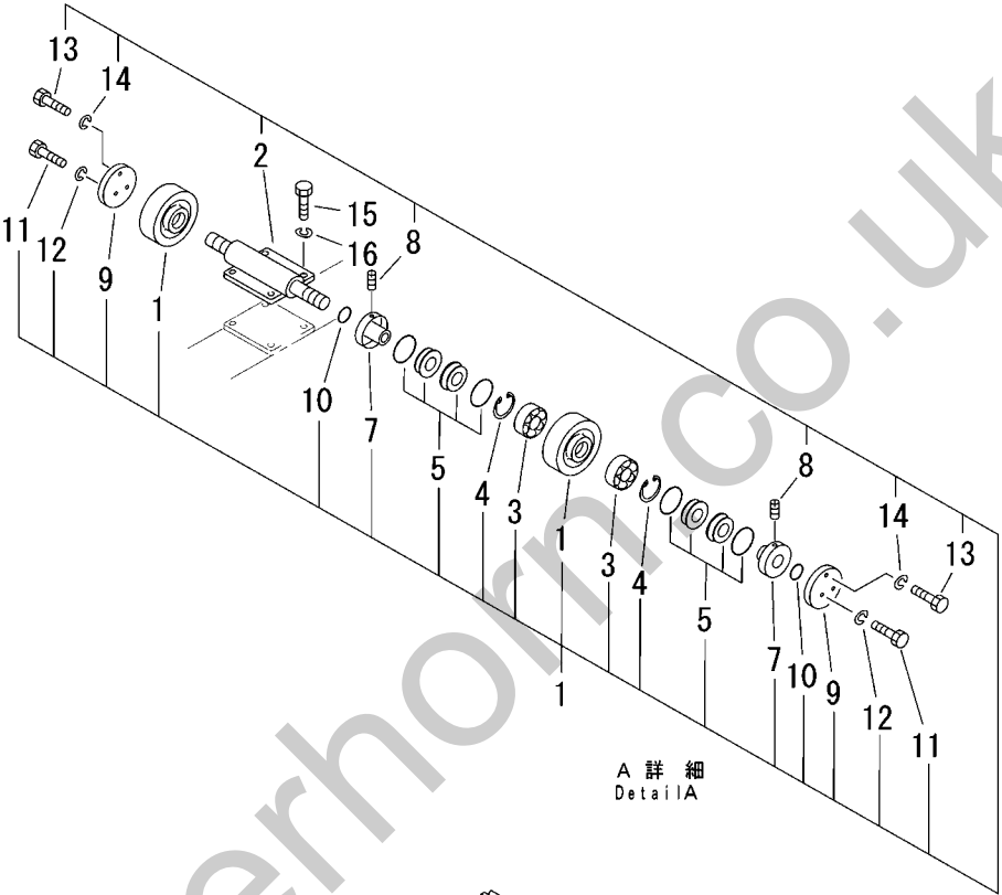
FIG..311 UNDER CARRIAGE RELATED PARTS (CARRIER ROLLER)
