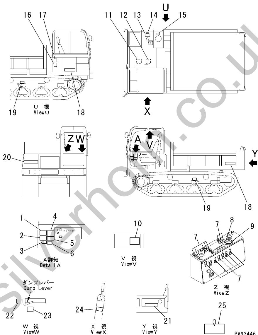
FIG.811 MARKS AND CAUTION PLATES (ENGLISH) (APPLICABLE TO CAB SPEC.)
