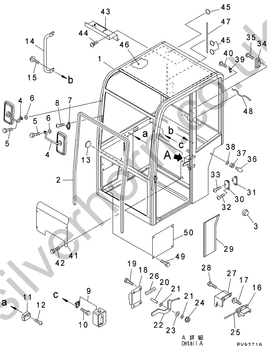
FIG..223 CAB ASSEMBLY (1/3) (CAB AND RELATED PARTS) (APPLICABLE TO CAB SPEC.)
