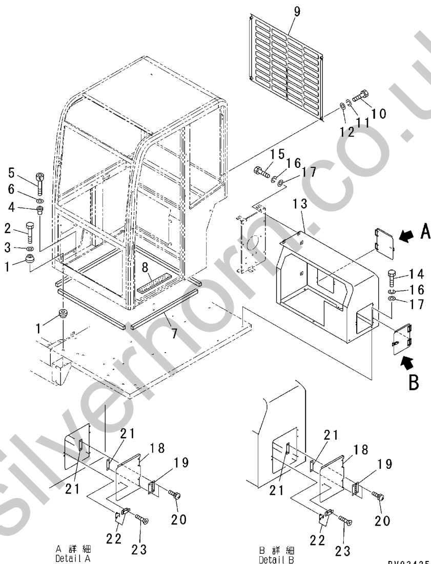
FIG..221 CAB RELATED PARTS (CAB AND MOUTING PARTS) (APPLICABLE TO CAB SPEC.)
