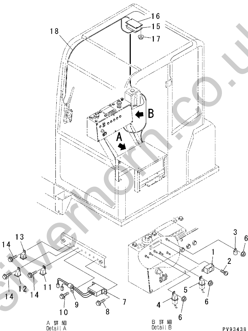
FIG..705 ELECTRICAL SYSTEM (CAB WIRING, BUZZER AND RELAY) (APPLICABLE TO CAB SPEC.)
