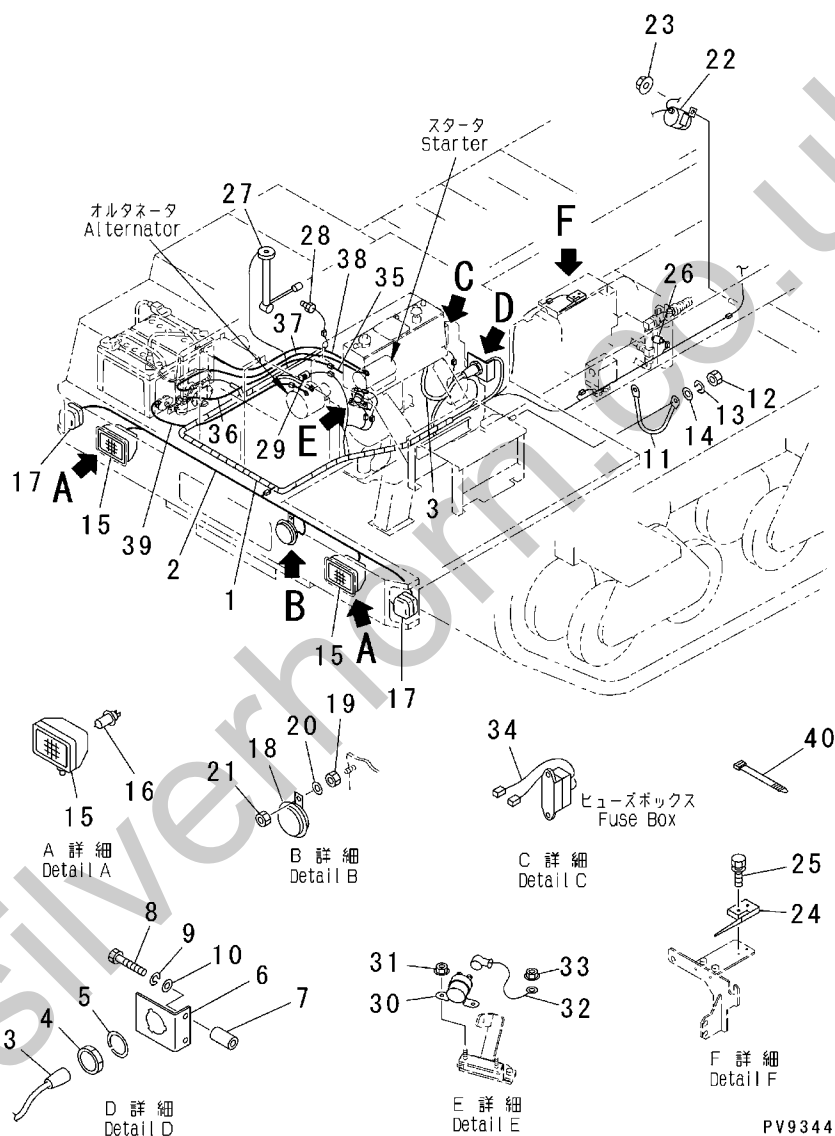
FIG..711 ELECTRICAL SYSTEM (CHASSIS WIRING HARNESS AND LAMPS)
