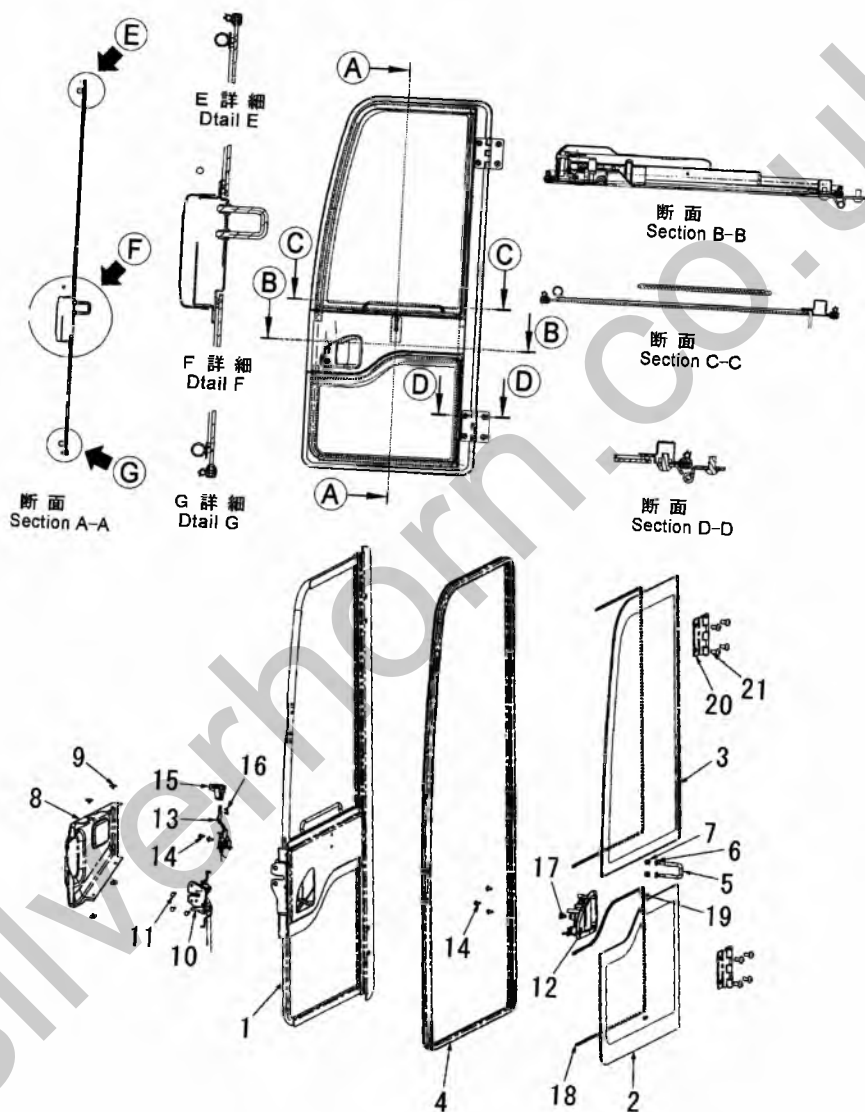
FIG.227 CAB (7/12) (DOOR GROUP)
