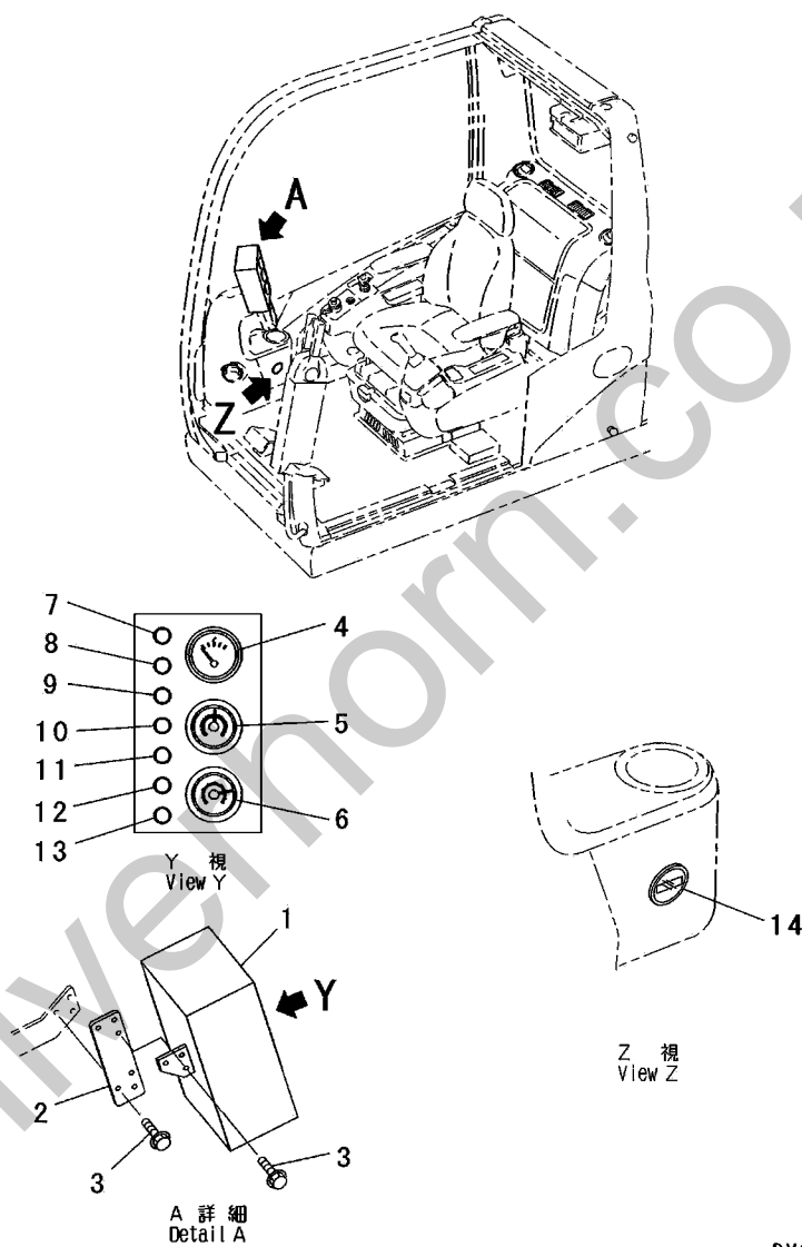
FIG. 701 ELECTRICAL SYSTEM (METER BOX IN CAB)
