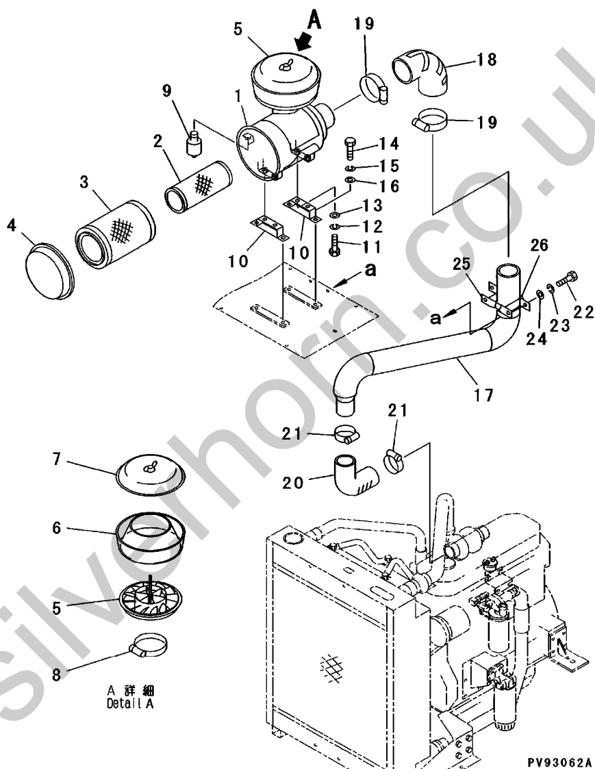
FIG.111 ENGINE RELATED PARTS(AIR INTAKE SYSTEM)
