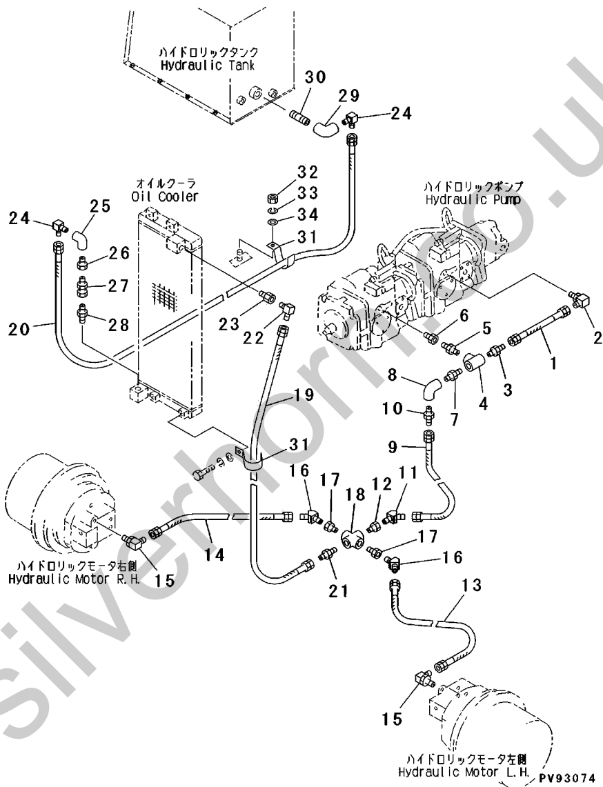
FIG.506 HYDRAULIC OIL PIPING (OIL COOLER AND DRAIN LINE) (EXCEPT JAPAN) (SERIAL NO.223183-223339)
