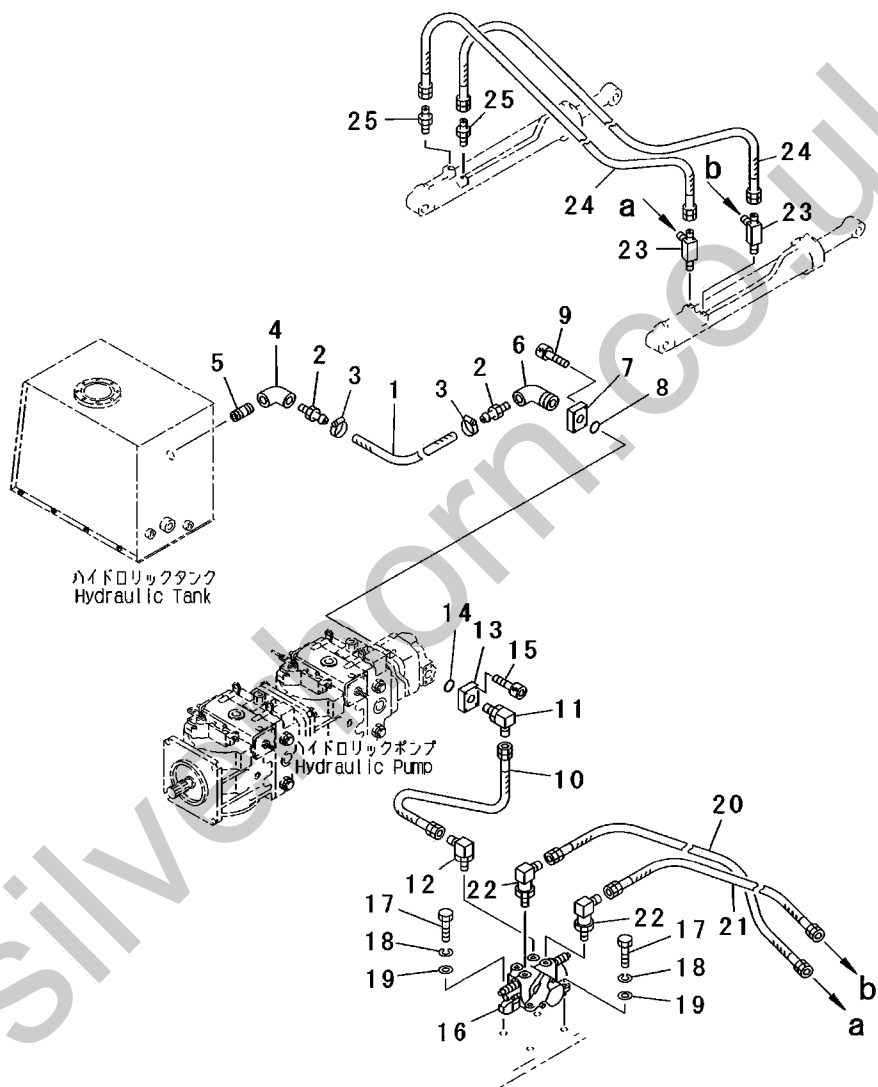
FIG.501A HYDRAULIC OIL PIPING (CONTROL VALVE AND DUMP CYLINDER LINE) (SERIAL NO.22340-)
