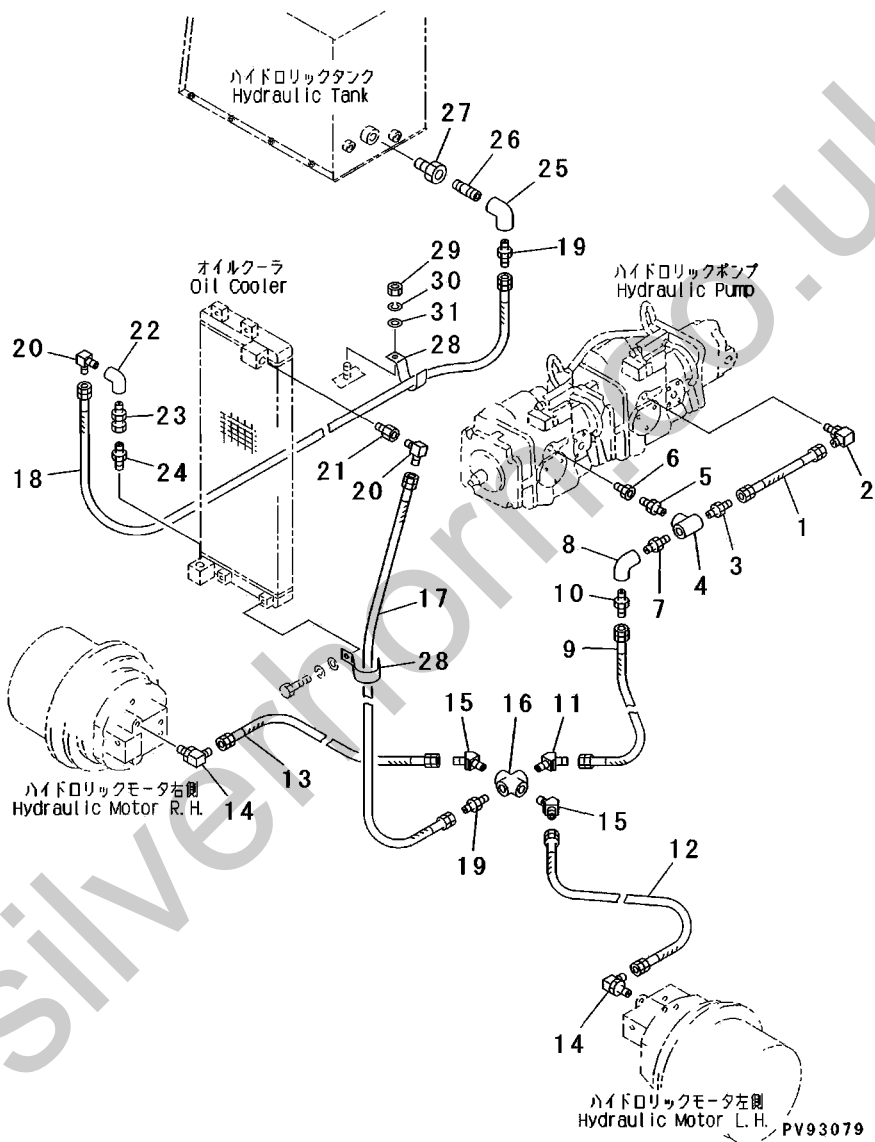
FIG.505 HYDRAULIC OIL PIPING (OIL COOLER AND DRAIN LINE) (SERIAL NO.223101-223182)
