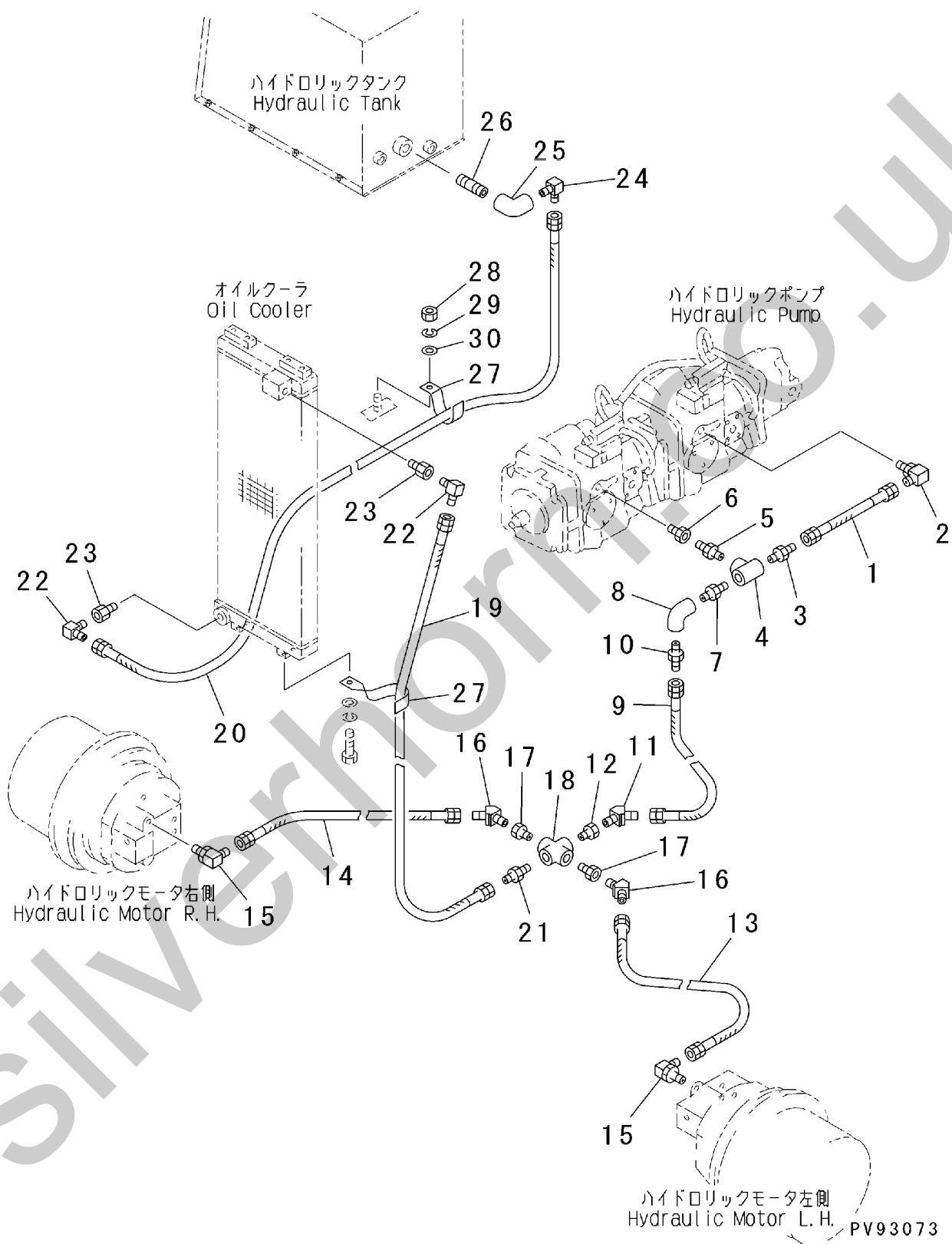
FIG.505A HYDRAULIC OIL PIPING (OIL COOLER AND DRAIN LINE) (FOR JAPAN) (SERIAL NO.223183-)
