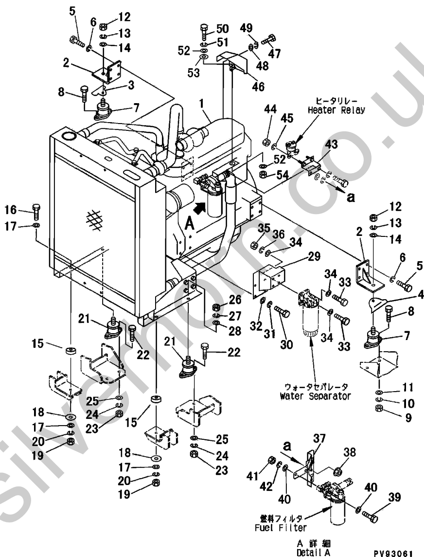
FIG.101 ENGINE RELATED PARTS (ENGINE MOUNTING PARTS AND RADIATOR)
