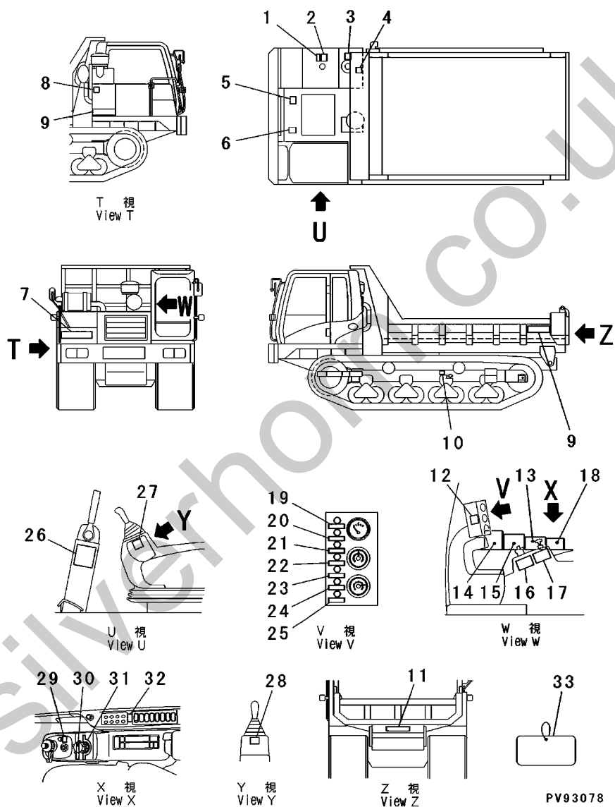
FIG.811 MARKS AND PLATES (ENGLISH) (SERIAL NO.223101-223344)
