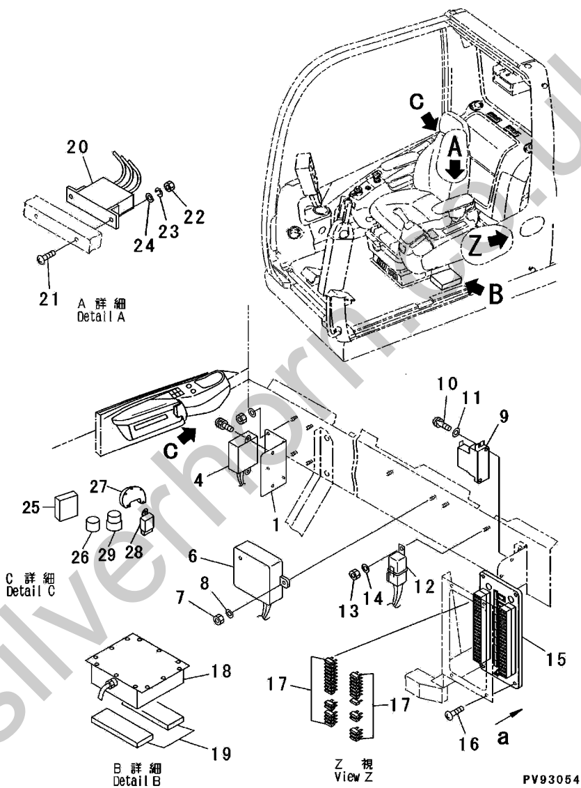
FIG.713 ELECTRICAL SYSTEM (RELAY AND FUSE BOX)
