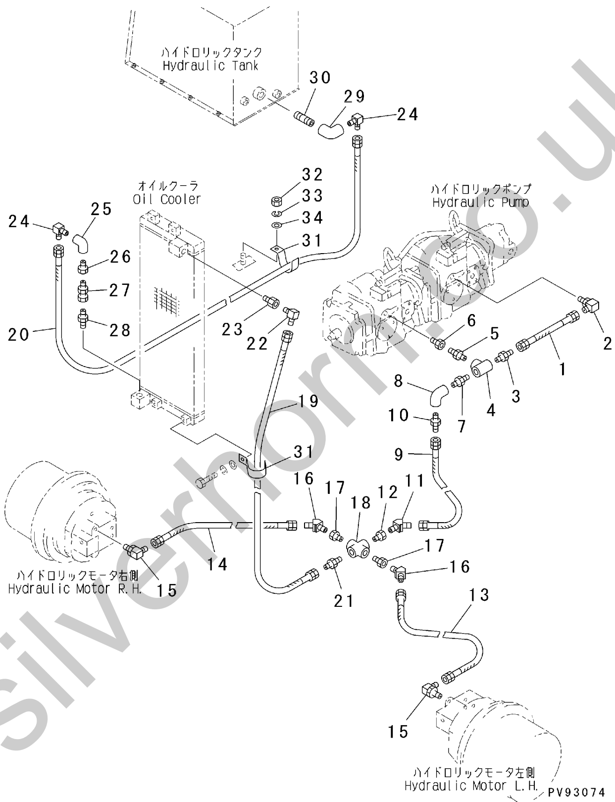
FIG.506 HYDRAULIC OIL PIPING (OIL COOLER AND DRAIN LINE) (EXCEPT JAPAN) (SERIAL NO.223183-)
