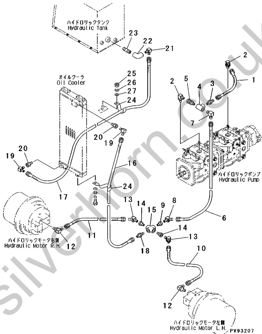
FIG. 505A HYDRAULIC OIL PIPING (OIL COOLER AND DRAIN LINE) (SERIAL NO.223340-223346)
