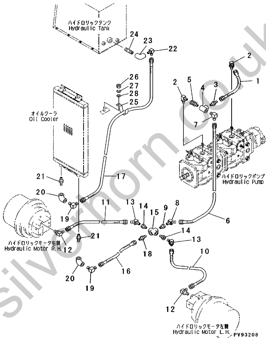
FIG. 505B HYDRAULIC OIL PIPING (OIL COOLER AND DRAIN LINE) (SERIAL NO.223347-)
