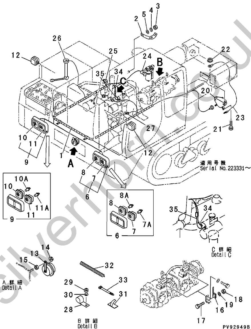
FIG.711 ELECTRICAL SYSTEM (WIRING HARNESS AND LAMPS)
