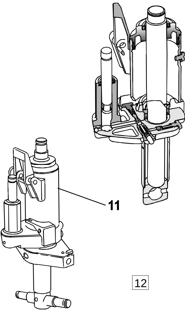
6400-013 Manual pump unit, jack [1997-02-18] Manuell hydraul, domkraft; Manuelle Hydraulikeinheit/Pumpe; Groupe hydraulique manuel, cric
