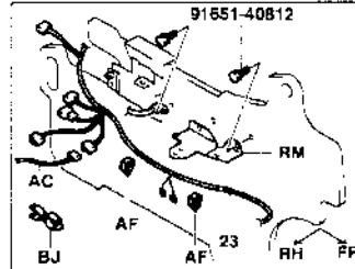
[FRONT PLATE,LH]
