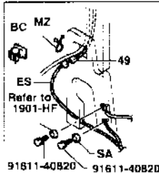
[LH PILLAR]
