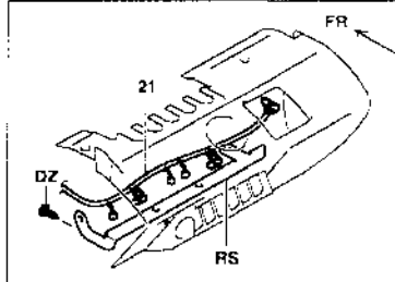
[REAR FRAME]
