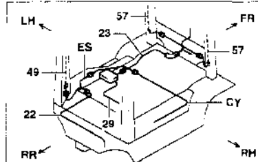
[FRONT PLATE,LH]
