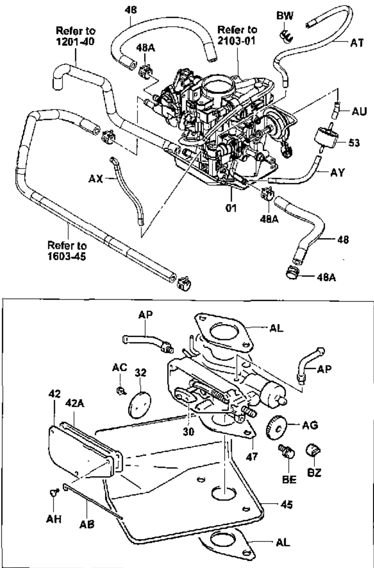
2105-091
