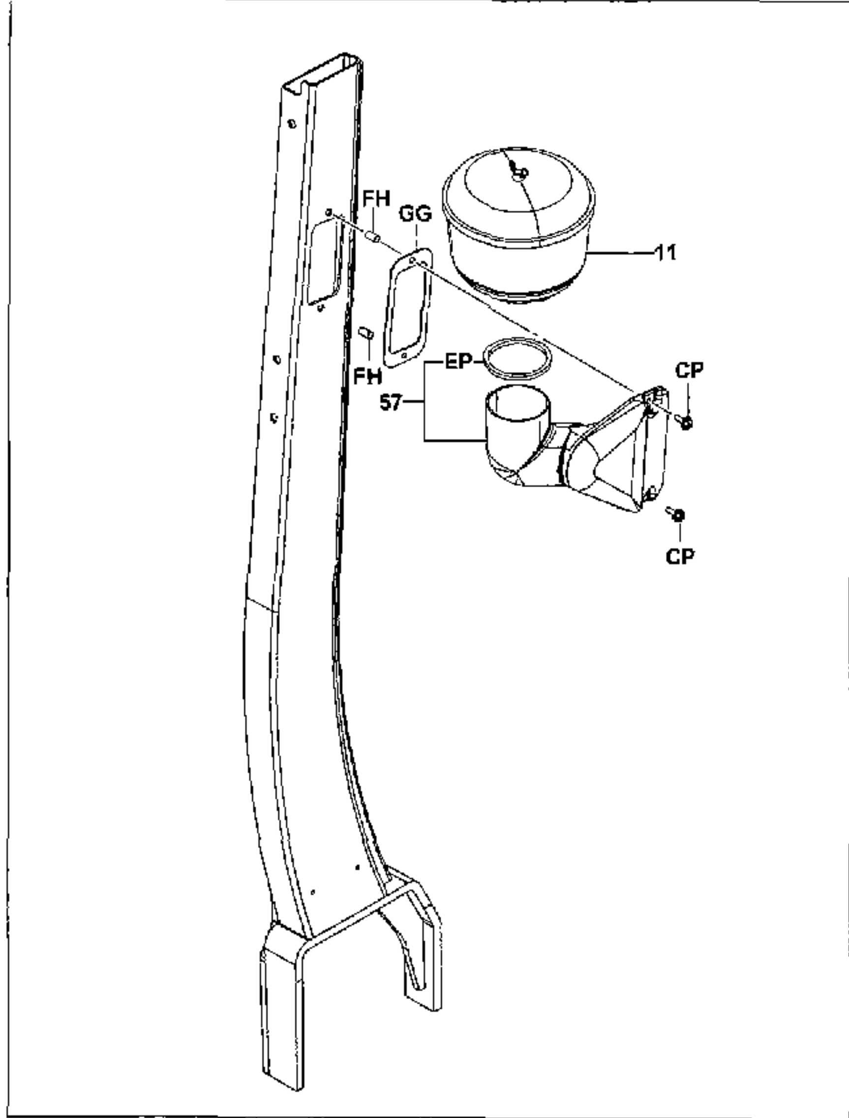
PRE-CLEANER
