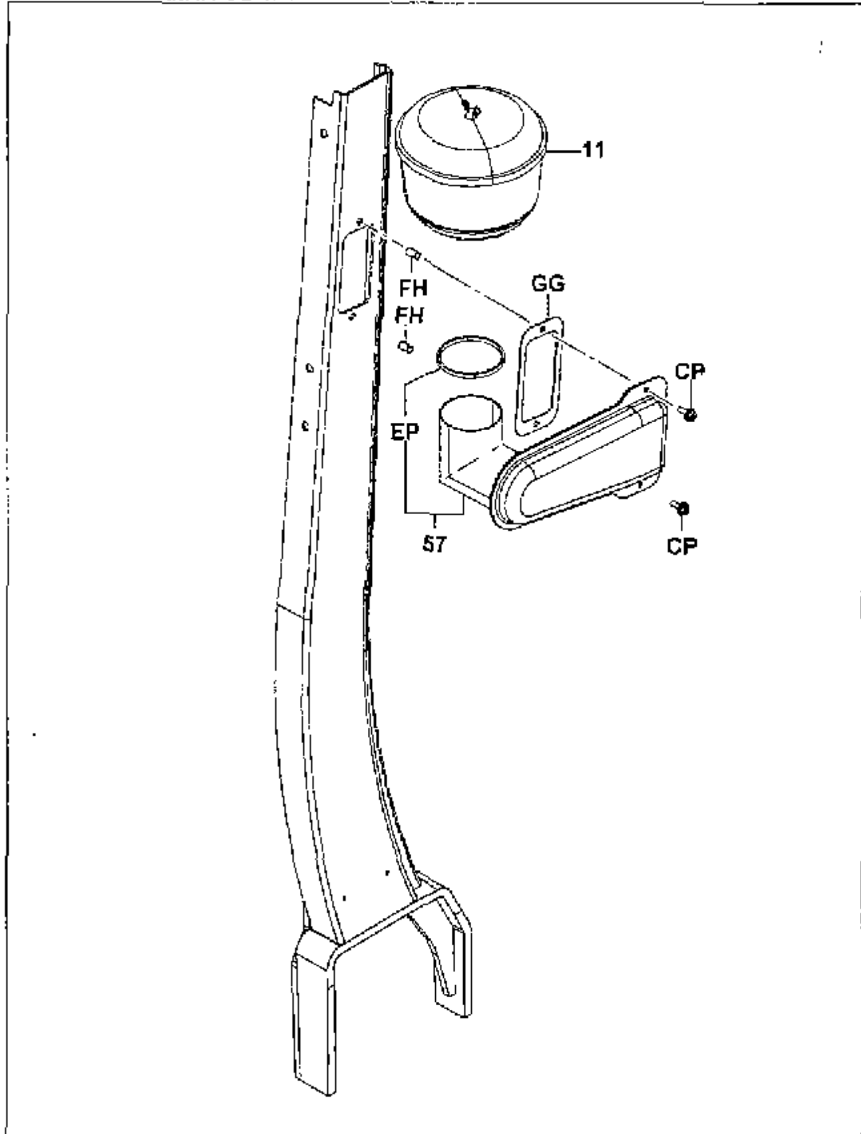
PRE-CLEANER,RR GLASS
