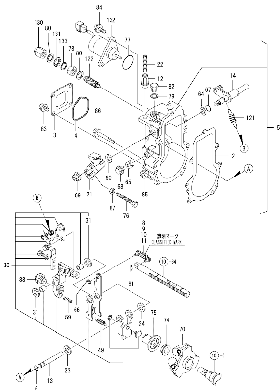
Fig.11. GOVERNOR
