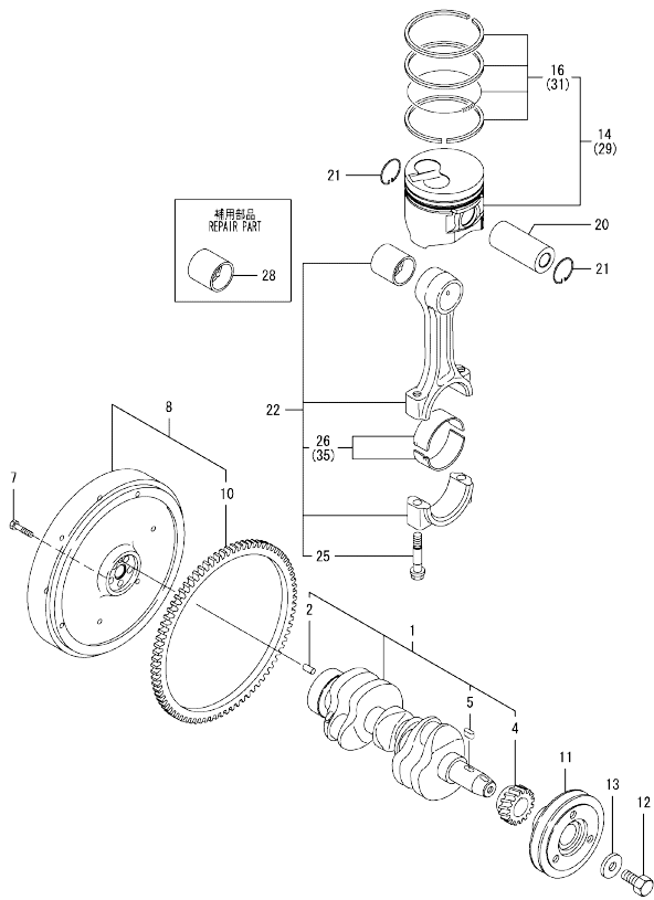
Fig.7. CRANKSHAFT & PISTON
