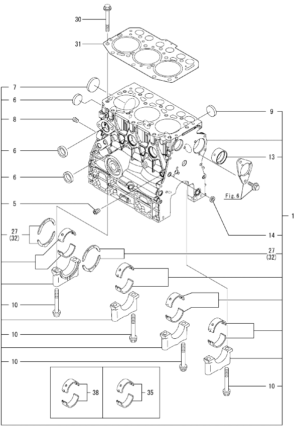
Fig.1. CYLINDER BLOCK
