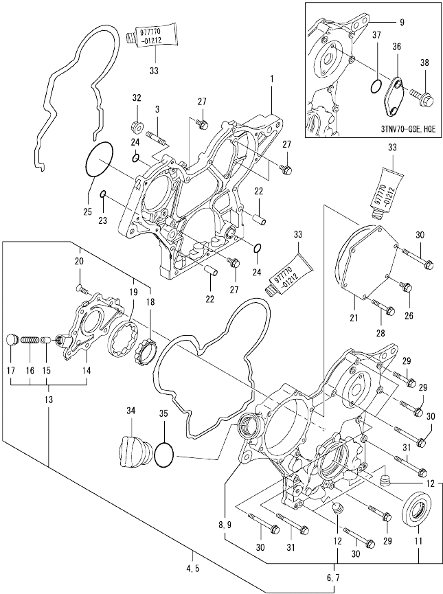
Fig.2. GEAR HOUSING
