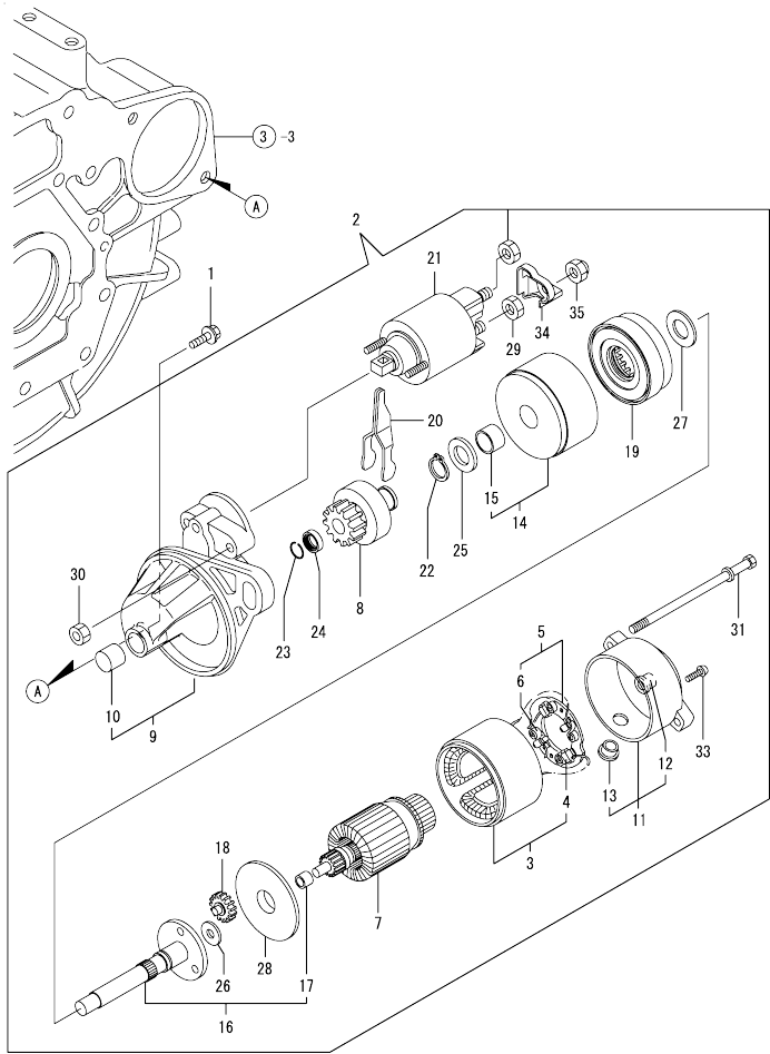
Fig.15. STARTER MOTOR
