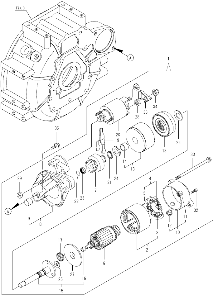
OCR10-M85800 3TNV70-GGEA Fig.15. STARTING MOTOR
