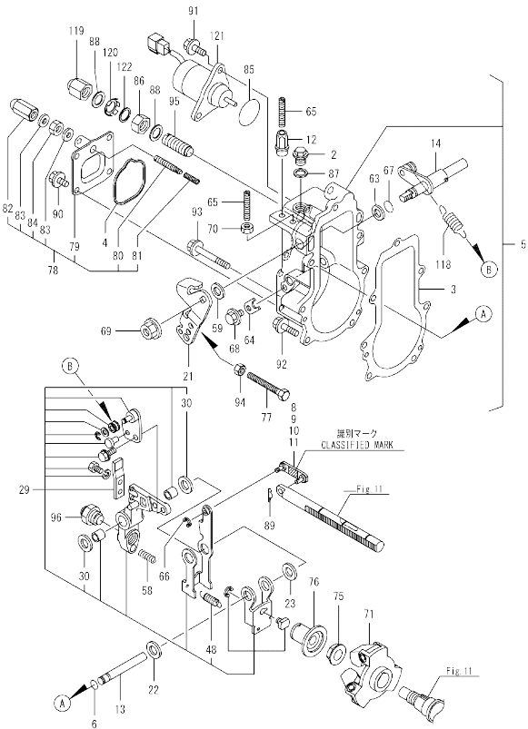
Fig.12. GOVERNOR
