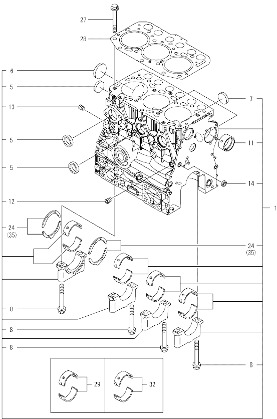
OCR10-M85800 3TNV70-GGEA Fig.1. CYLINDER BLOCK
