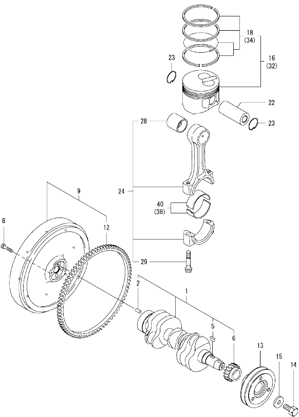
Fig.6. CRANKSHAFT & PISTON
