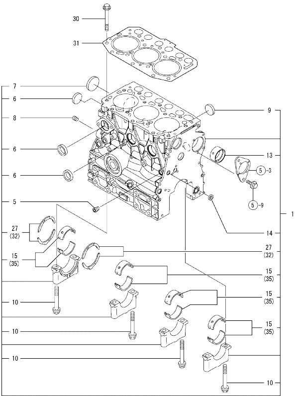
Fig.1. CYLINDER BLOCK
