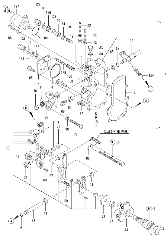
Fig.10. GOVERNOR
