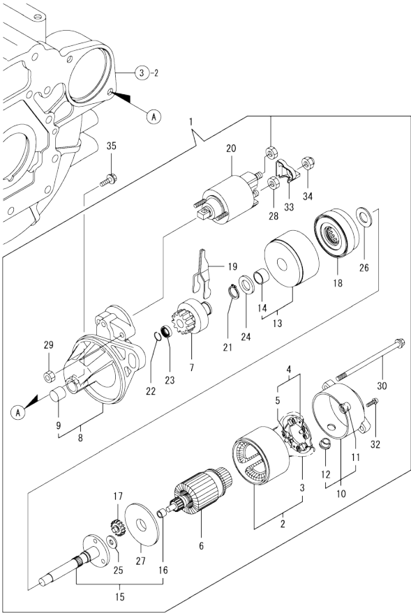
Fig.15. STARTING MOTOR
