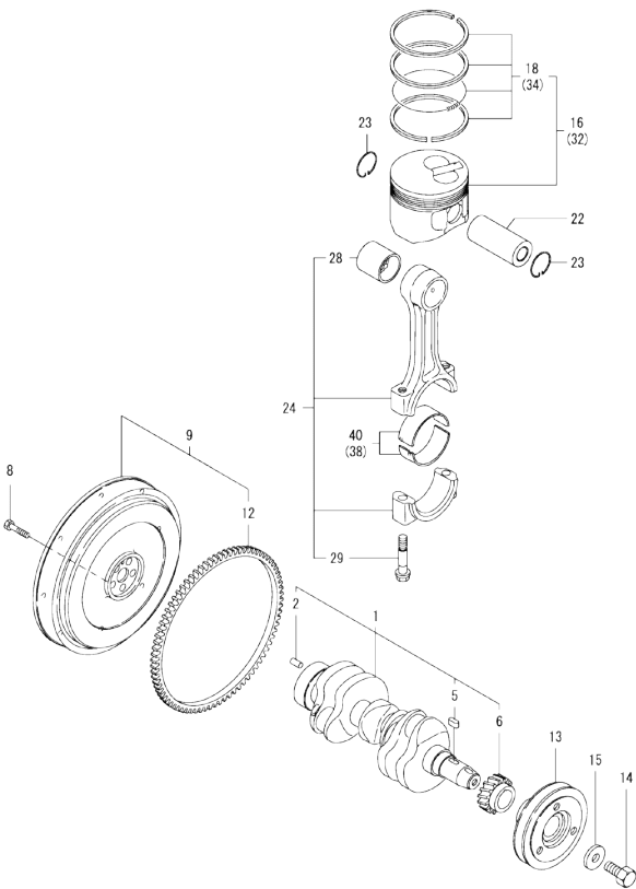
Fig.7. CRANKSHAFT & PISTON
