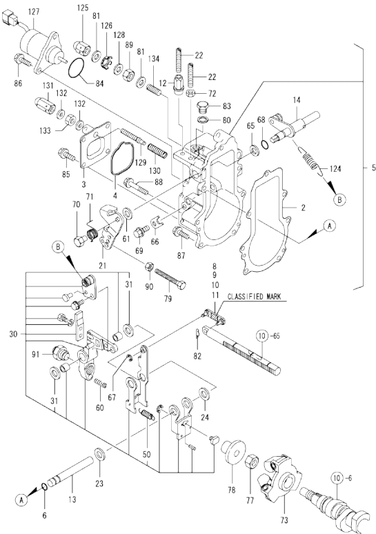
Fig.11. GOVERNOR
