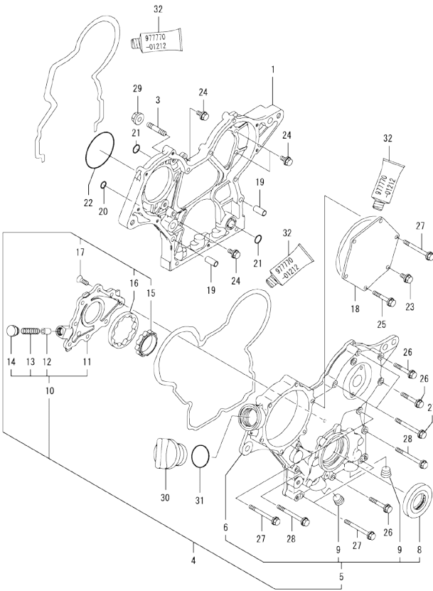
Fig.2. GEAR HOUSING
