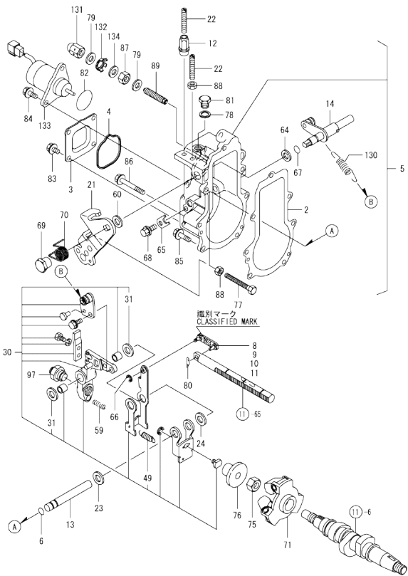
Fig.12. GOVERNOR
