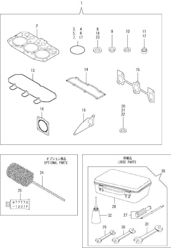
Fig.17. GASKET SET & TOOLS
