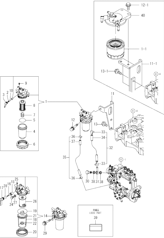
Fig.14. FUEL LINE
