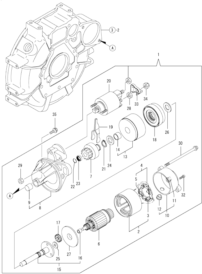
Fig.15. STARTING MOTOR
