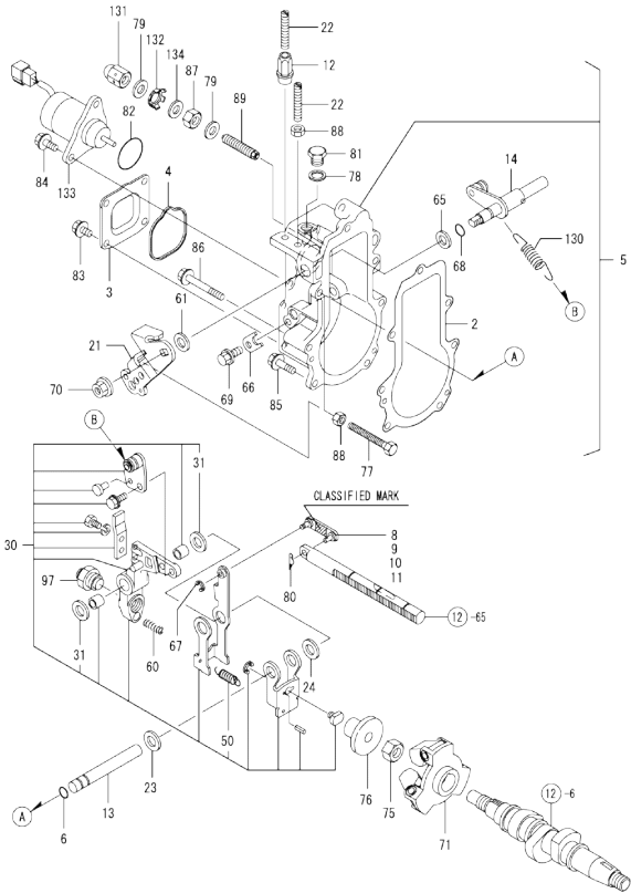
Fig.13. GOVERNOR
