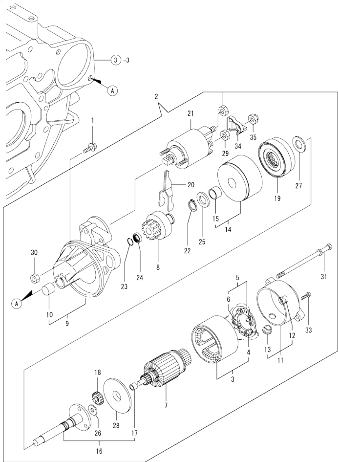
Fig.15. STARTER MOTOR
