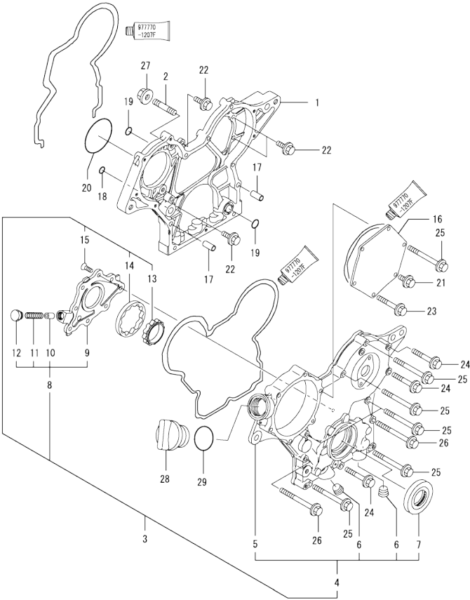
Fig.2. GEAR HOUSING
