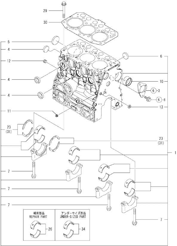
Fig.1. CYLINDER BLOCK
