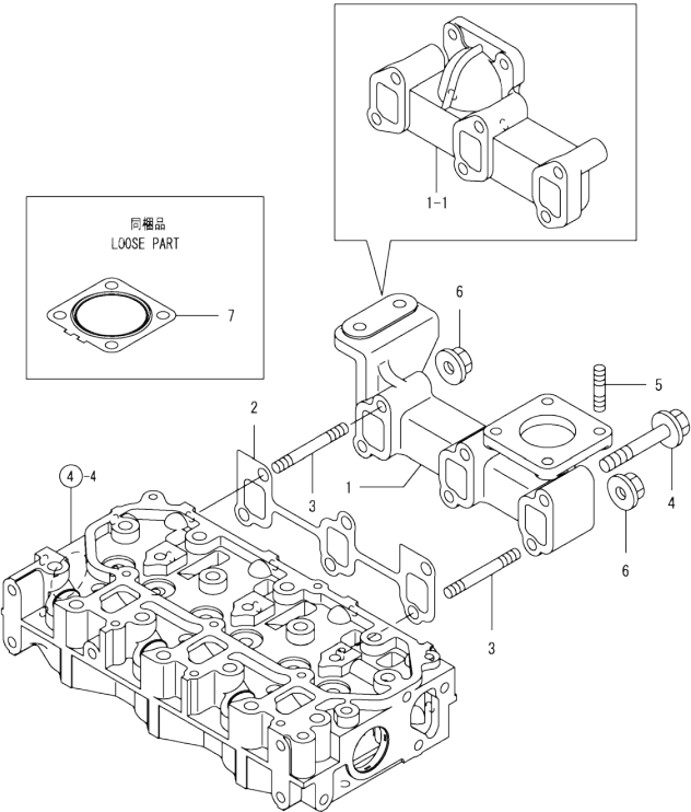
Fig.5. EXHAUST MANIFOLD
