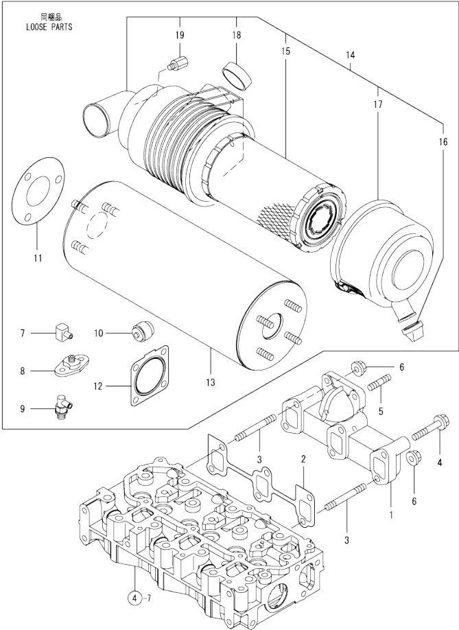
Fig.5. EXHAUST MANIFOLD & AIR CLEANER
