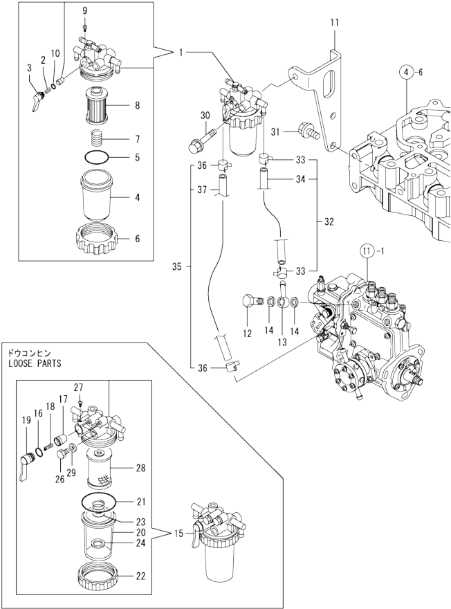
Fig.14. FUEL LINE
