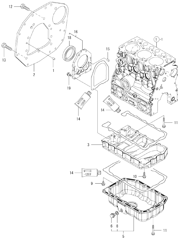
Fig.3. MOUNTING FLANGE & OIL SUMP
