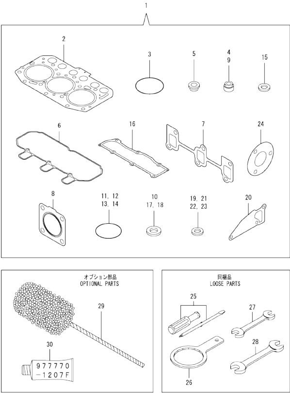
Fig.20. GASKET SET
