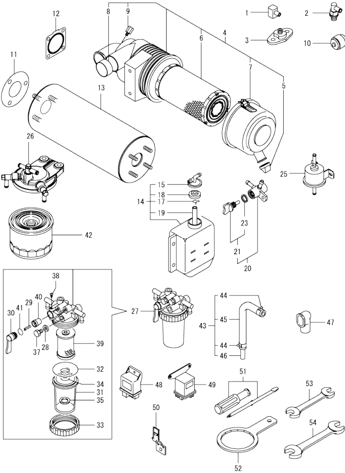
OCD50-M02670 ENGINE Fig.16. ACCESSORY
