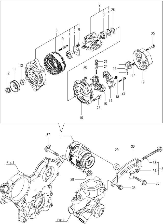
OCD50-M02670 ENGINE Fig.15. GENERATOR
