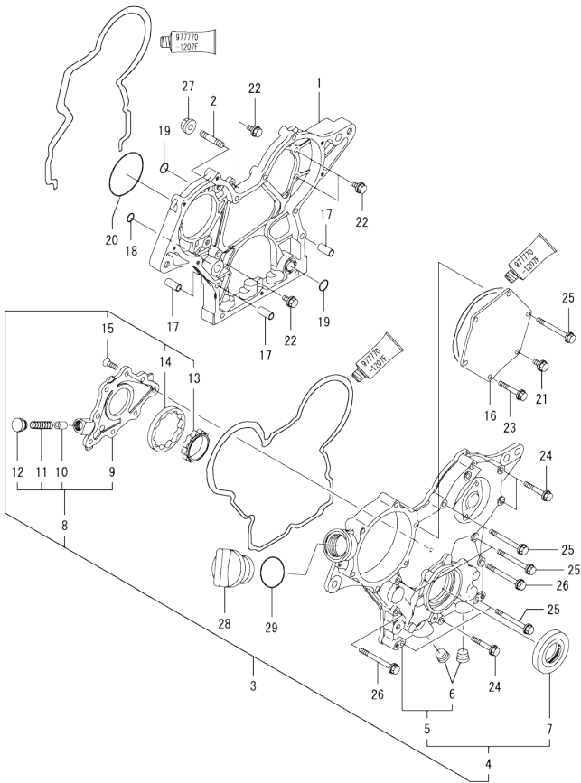
0CW10-M50800 3TNV70-QIKX Fig.2. GEAR HOUSING
