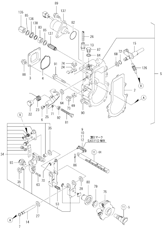
Fig.12. GOVERNOR
