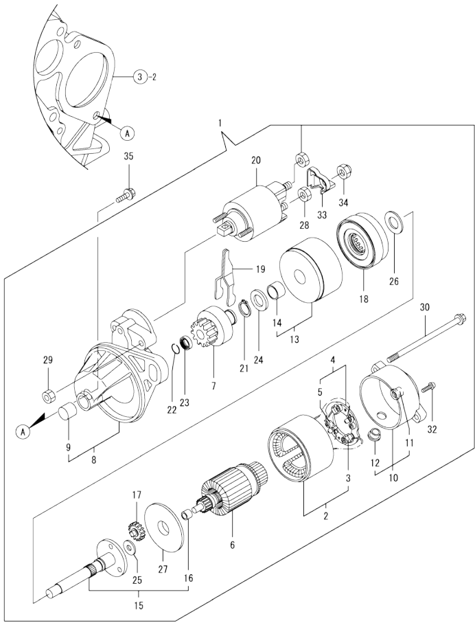
0CW10-M50800 3TNV70-QIKX Fig.15. STARTING MOTOR
