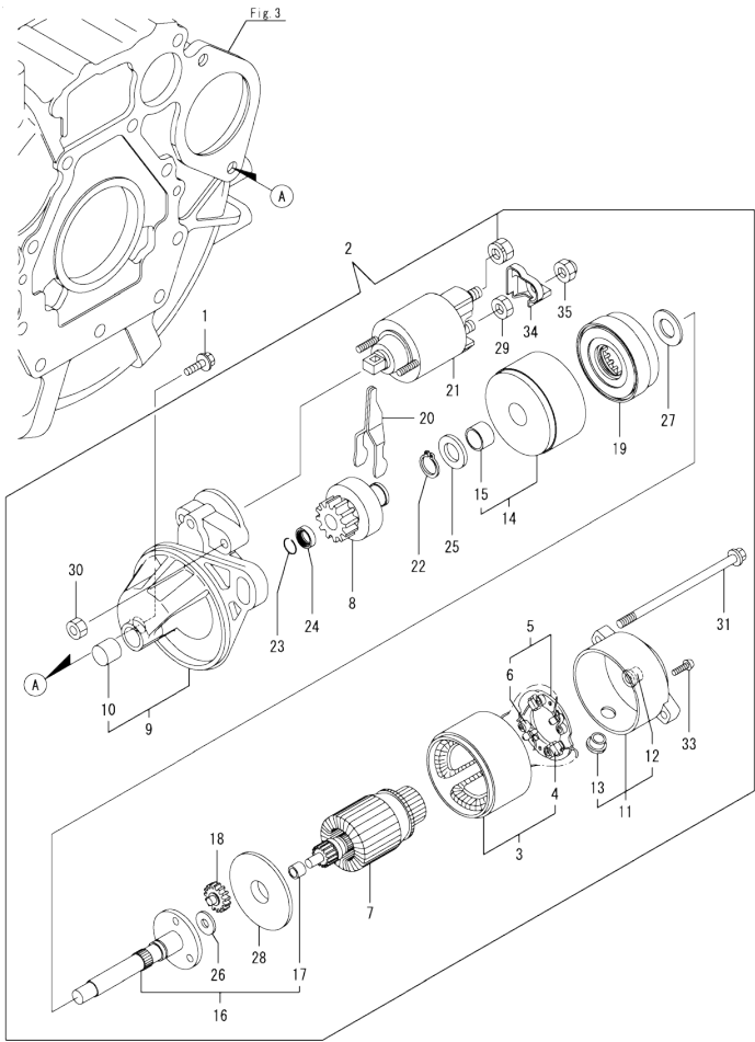
Fig.15. STARTER MOTOR
