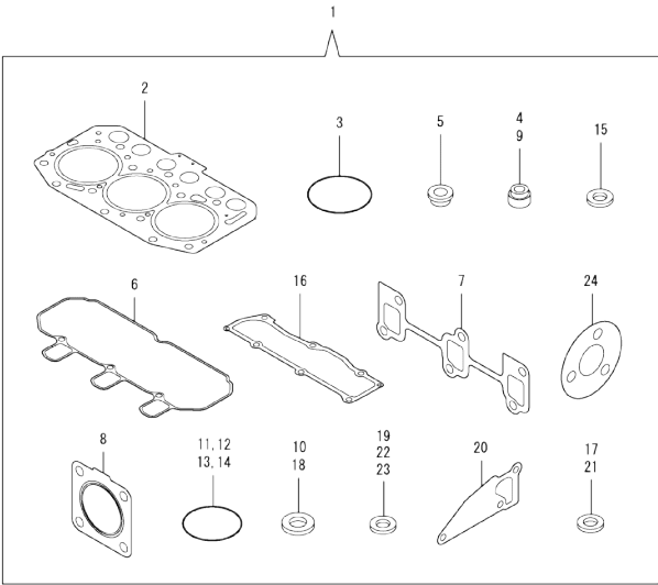
Fig.17. GASKET SET
