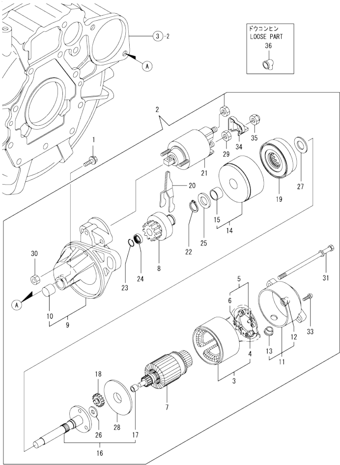
Fig.15. STARTING MOTOR
