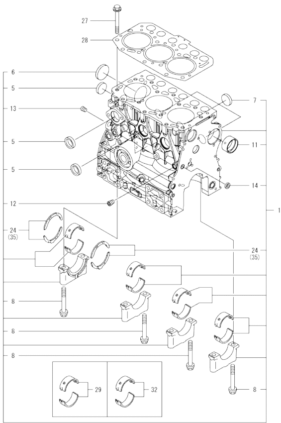
Fig.1. CYLINDER BLOCK
