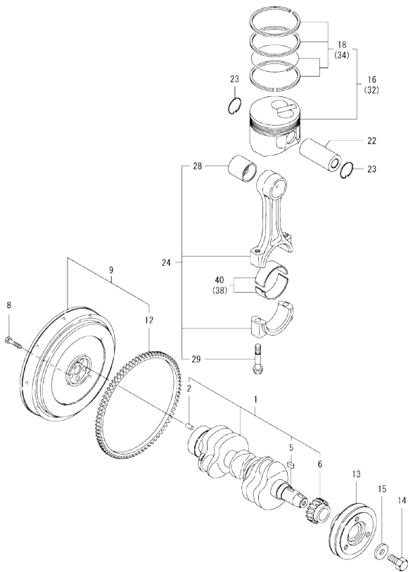
Fig.7. CRANKSHAFT & PISTON
