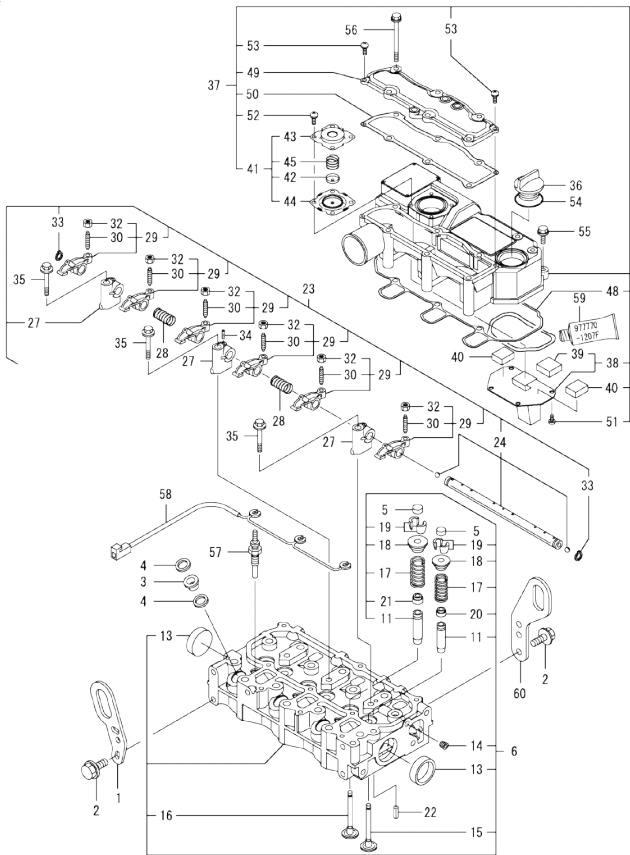
Fig.4. CYLINDER HEAD & BONNE
