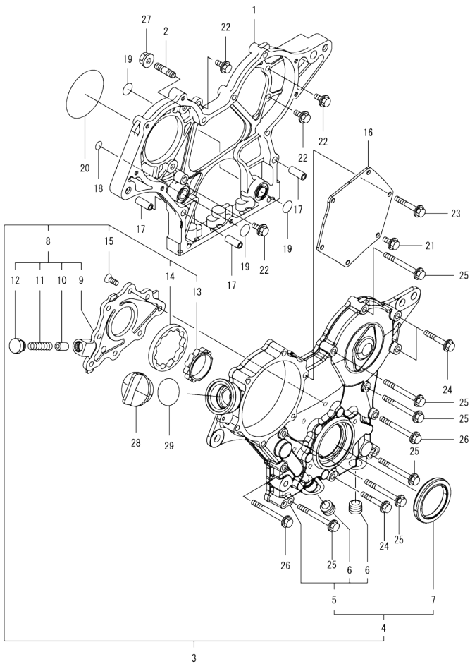
Fig.2. GEAR HOUSING
