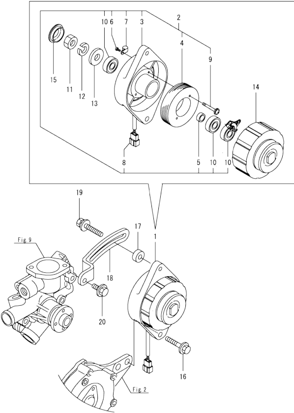
OCD50-M04480 ENGINE Fig.15. GENERATOR
